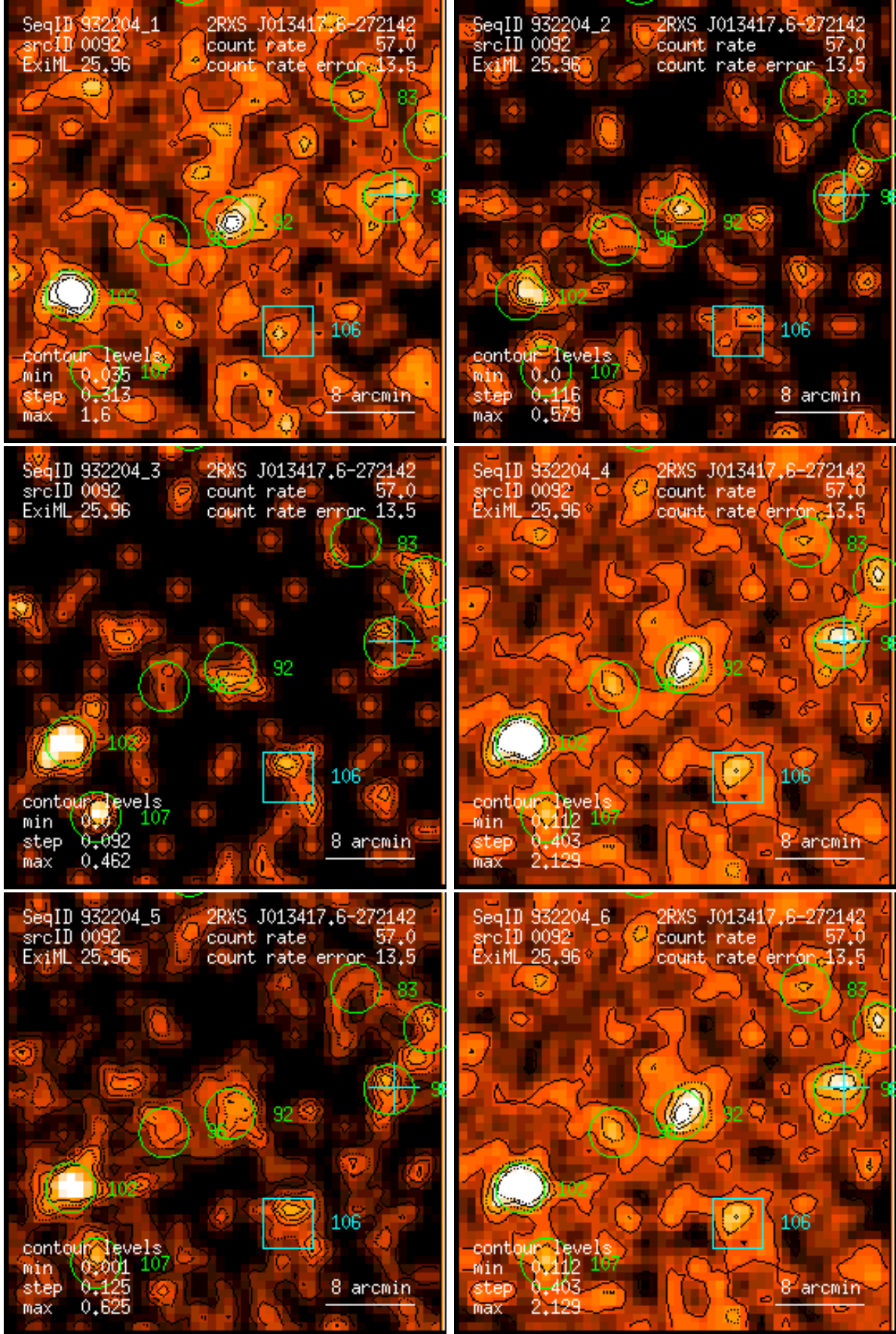
Figure 92: RASS 932204: detection 0092: band rate images, Gaussian filter: (1) PSPC channels 11 – 41, (2) 52 – 90, (3) 91 – 201, (4) 11 – 235, (5) 52 – 201, (6) 11 – 201. Broad band rates in counts/ks. Band rate contour levels in counts/ks/arcmin 2 .
