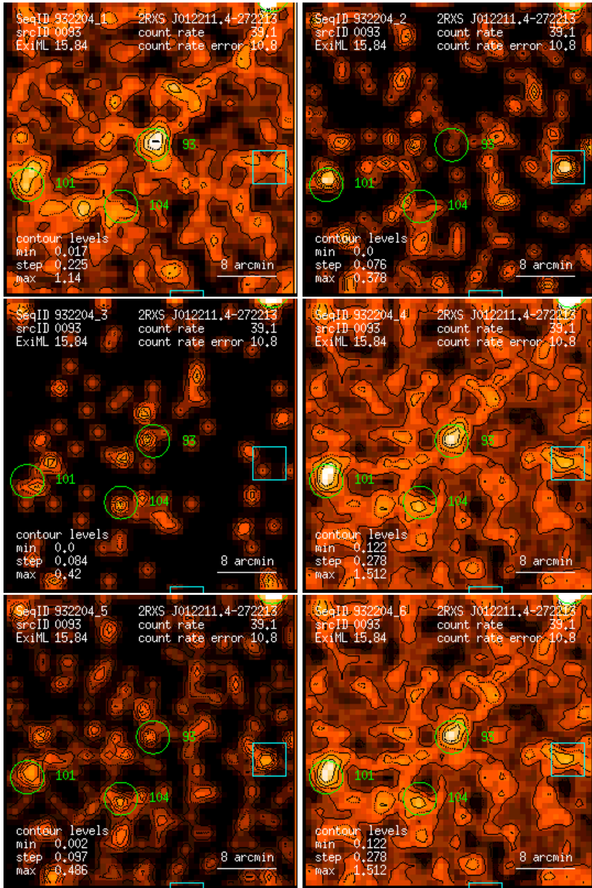
Figure 93: RASS 932204: detection 0093: band rate images, Gaussian filter: (1) PSPC channels 11 – 41, (2) 52 – 90, (3) 91 – 201, (4) 11 – 235, (5) 52 – 201, (6) 11 – 201. Broad band rates in counts/ks. Band rate contour levels in counts/ks/arcmin 2 .
