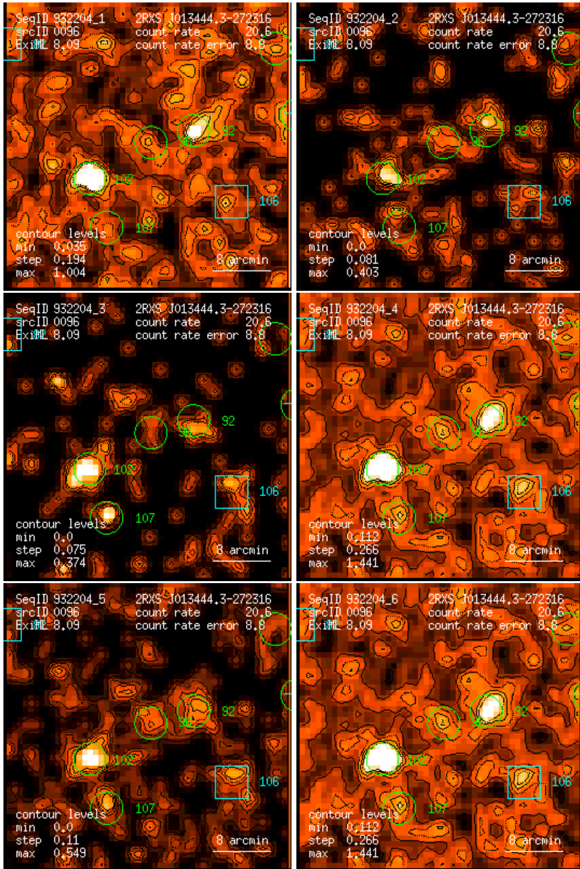
Figure 96: RASS 932204: detection 0096: band rate images, Gaussian filter: (1) PSPC channels 11 – 41, (2) 52 – 90, (3) 91 – 201, (4) 11 – 235, (5) 52 – 201, (6) 11 – 201. Broad band rates in counts/ks. Band rate contour levels in counts/ks/arcmin 2 .
