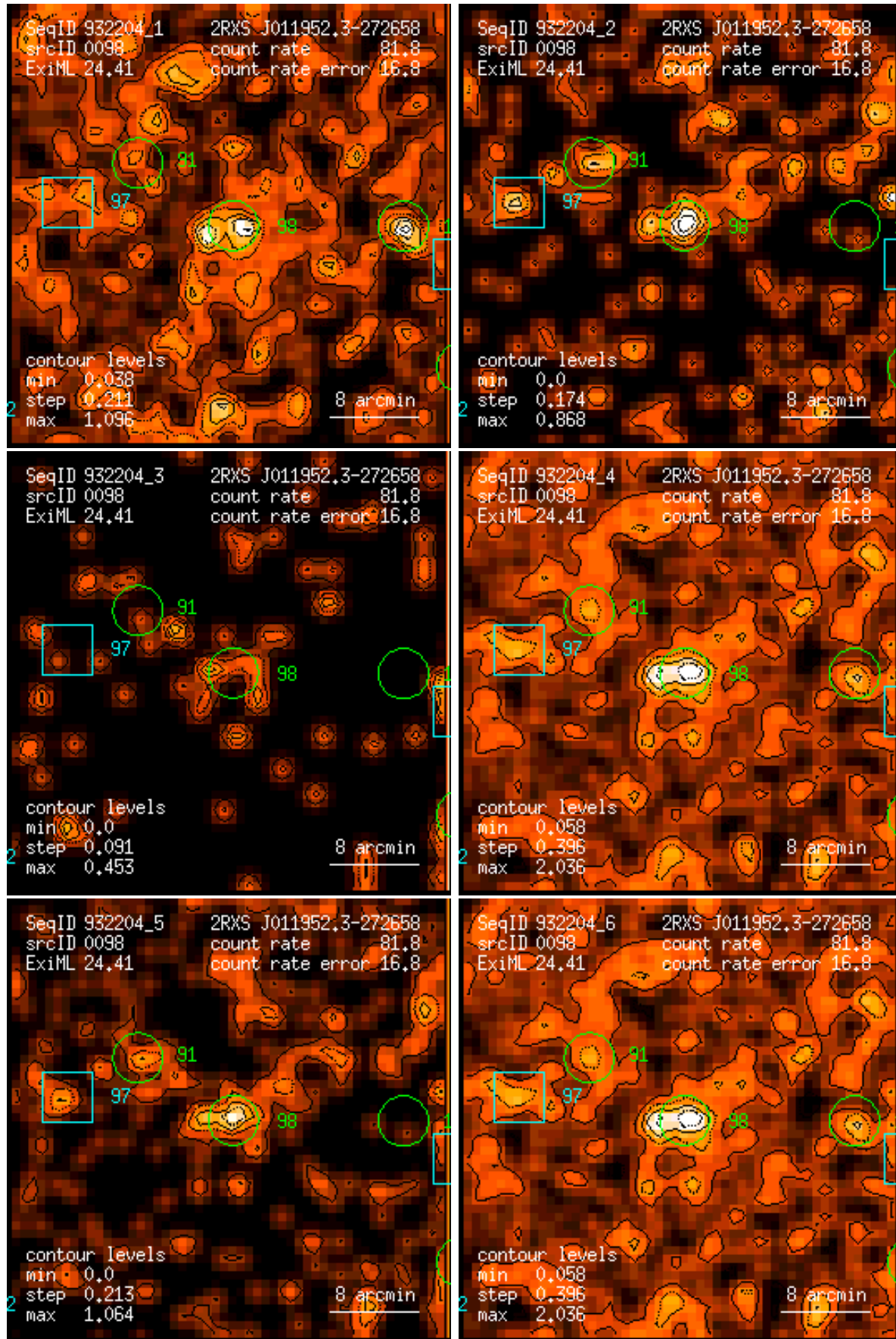
Figure 98: RASS 932204: detection 0098: band rate images, Gaussian filter: (1) PSPC channels 11 – 41, (2) 52 – 90, (3) 91 – 201, (4) 11 – 235, (5) 52 – 201, (6) 11 – 201. Broad band rates in counts/ks. Band rate contour levels in counts/ks/arcmin 2 .
