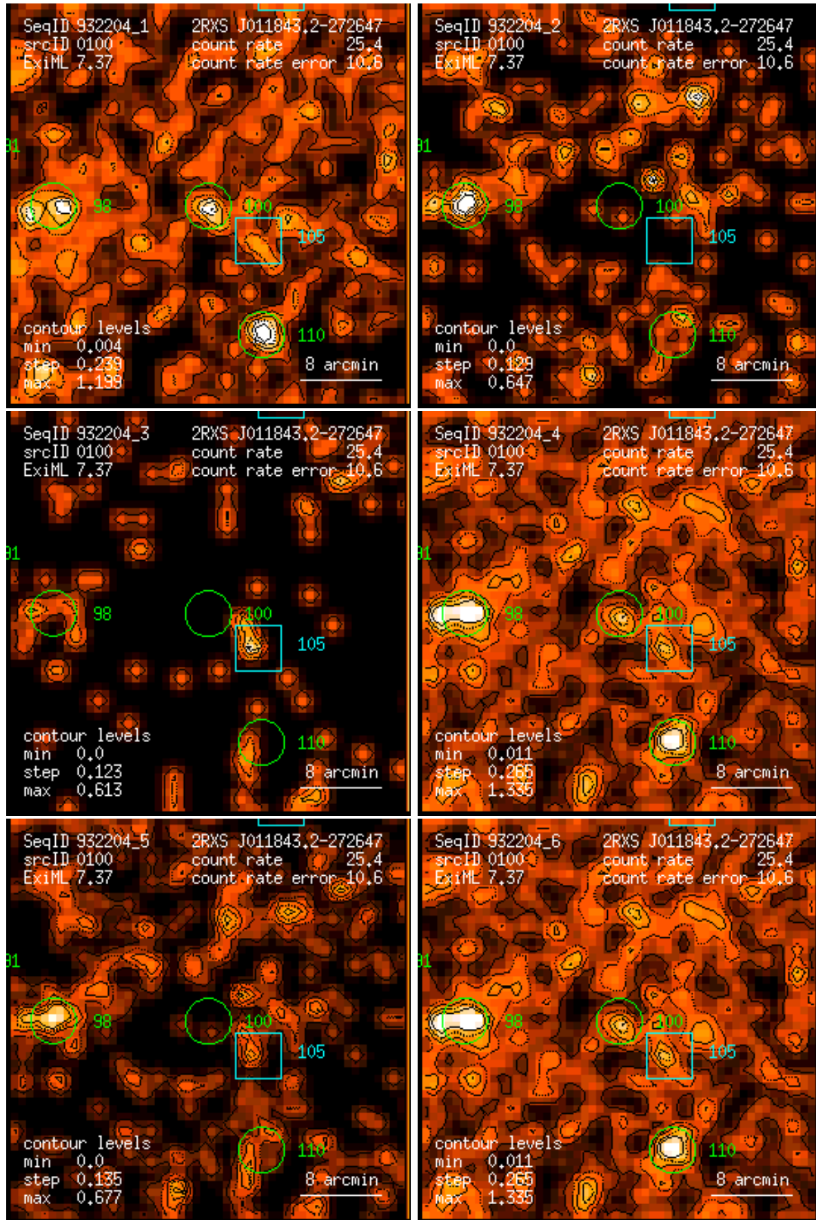
Figure 100: RASS 932204: detection 0100: band rate images, Gaussian filter: (1) PSPC channels 11 – 41, (2) 52 – 90, (3) 91 – 201, (4) 11 – 235, (5) 52 – 201, (6) 11 – 201. Broad band rates in counts/ks. Band rate contour levels in counts/ks/arcmin 2 .
