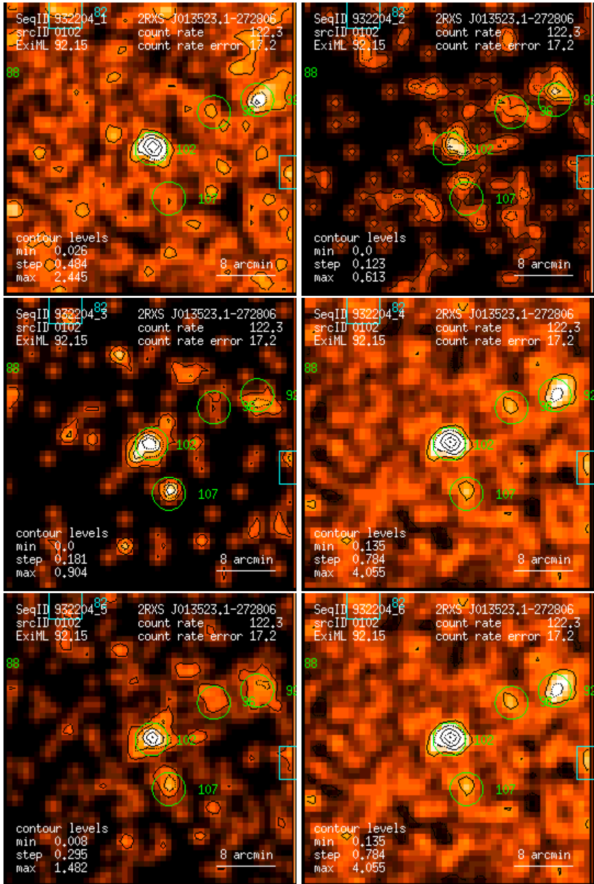
Figure 102: RASS 932204: detection 0102: band rate images, Gaussian filter: (1) PSPC channels 11 – 41, (2) 52 – 90, (3) 91 – 201, (4) 11 – 235, (5) 52 – 201, (6) 11 – 201. Broad band rates in counts/ks. Band rate contour levels in counts/ks/arcmin 2 .
