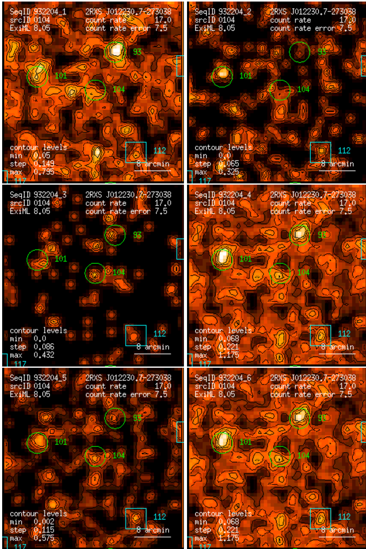
Figure 104: RASS 932204: detection 0104: band rate images, Gaussian filter: (1) PSPC channels 11 – 41, (2) 52 – 90, (3) 91 – 201, (4) 11 – 235, (5) 52 – 201, (6) 11 – 201. Broad band rates in counts/ks. Band rate contour levels in counts/ks/arcmin 2 .
