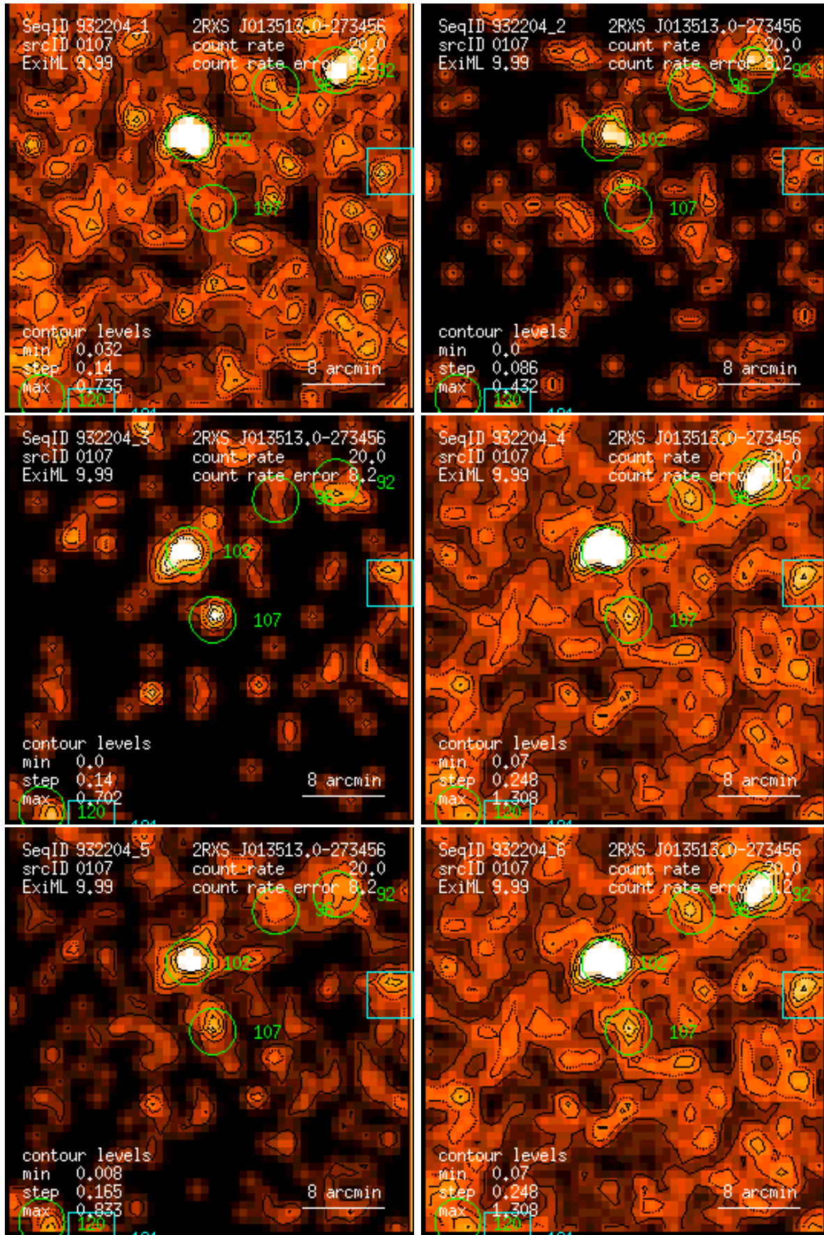
Figure 107: RASS 932204: detection 0107: band rate images, Gaussian filter: (1) PSPC channels 11 – 41, (2) 52 – 90, (3) 91 – 201, (4) 11 – 235, (5) 52 – 201, (6) 11 – 201. Broad band rates in counts/ks. Band rate contour levels in counts/ks/arcmin 2 .
