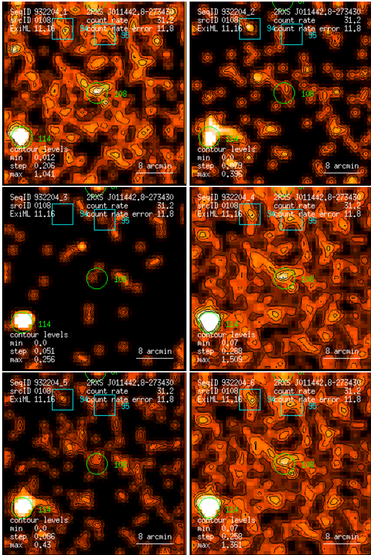
Figure 108: RASS 932204: detection 0108: band rate images, Gaussian filter: (1) PSPC channels 11 – 41, (2) 52 – 90, (3) 91 – 201, (4) 11 – 235, (5) 52 – 201, (6) 11 – 201. Broad band rates in counts/ks. Band rate contour levels in counts/ks/arcmin 2 .
