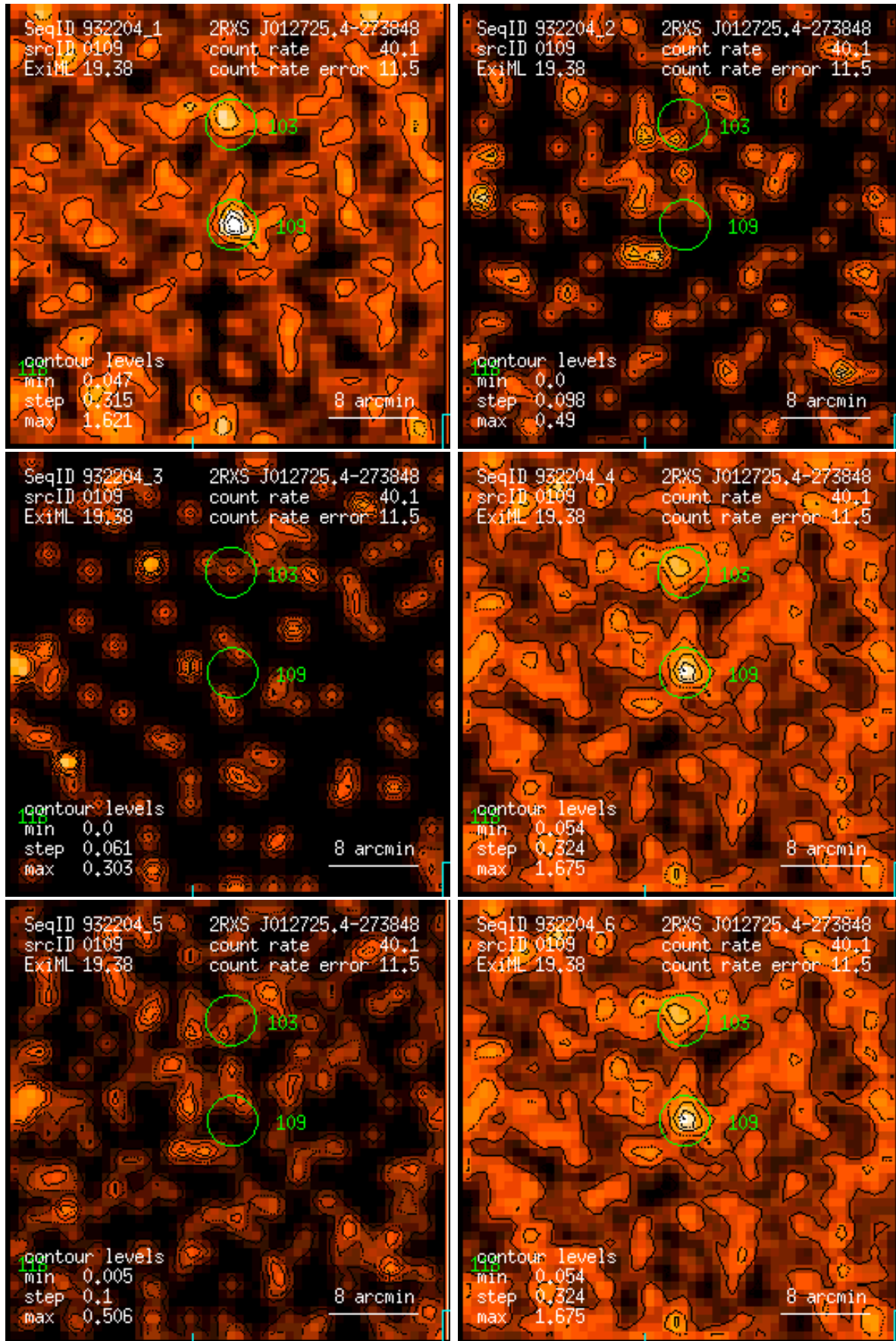
Figure 109: RASS 932204: detection 0109: band rate images, Gaussian filter: (1) PSPC channels 11 – 41, (2) 52 – 90, (3) 91 – 201, (4) 11 – 235, (5) 52 – 201, (6) 11 – 201. Broad band rates in counts/ks. Band rate contour levels in counts/ks/arcmin 2 .
