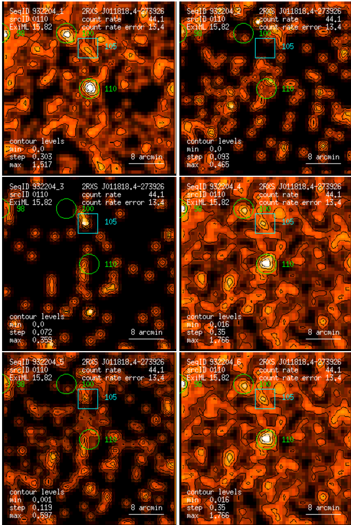
Figure 110: RASS 932204: detection 0110: band rate images, Gaussian filter: (1) PSPC channels 11 – 41, (2) 52 – 90, (3) 91 – 201, (4) 11 – 235, (5) 52 – 201, (6) 11 – 201. Broad band rates in counts/ks. Band rate contour levels in counts/ks/arcmin 2 .
