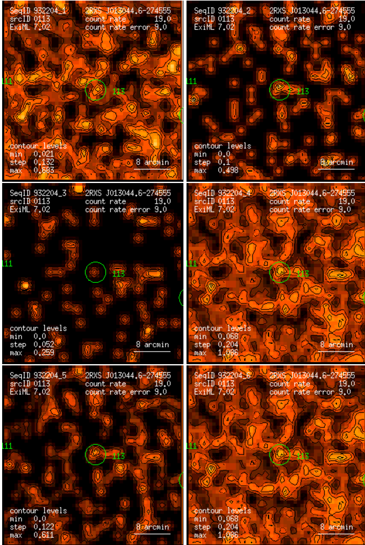
Figure 113: RASS 932204: detection 0113: band rate images, Gaussian filter: (1) PSPC channels 11 – 41, (2) 52 – 90, (3) 91 – 201, (4) 11 – 235, (5) 52 – 201, (6) 11 – 201. Broad band rates in counts/ks. Band rate contour levels in counts/ks/arcmin 2 .
