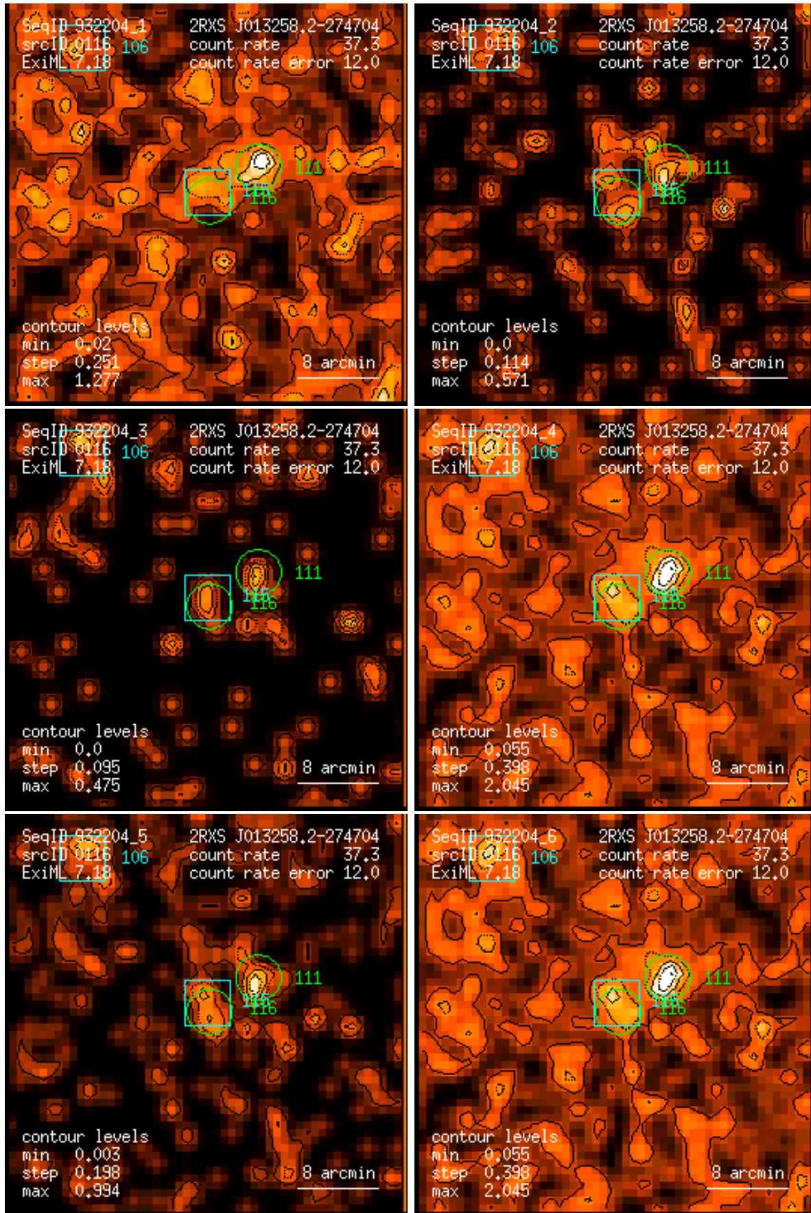
Figure 116: RASS 932204: detection 0116: band rate images, Gaussian filter: (1) PSPC channels 11 – 41, (2) 52 – 90, (3) 91 – 201, (4) 11 – 235, (5) 52 – 201, (6) 11 – 201. Broad band rates in counts/ks. Band rate contour levels in counts/ks/arcmin 2 .
