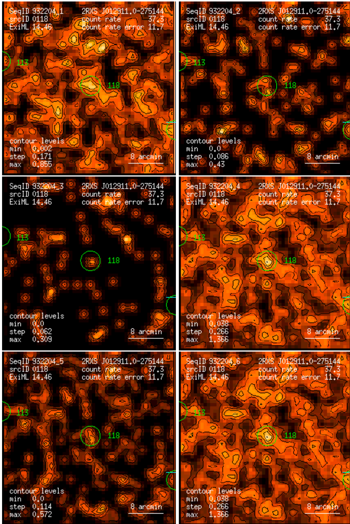
Figure 118: RASS 932204: detection 0118: band rate images, Gaussian filter: (1) PSPC channels 11 – 41, (2) 52 – 90, (3) 91 – 201, (4) 11 – 235, (5) 52 – 201, (6) 11 – 201. Broad band rates in counts/ks. Band rate contour levels in counts/ks/arcmin 2 .
