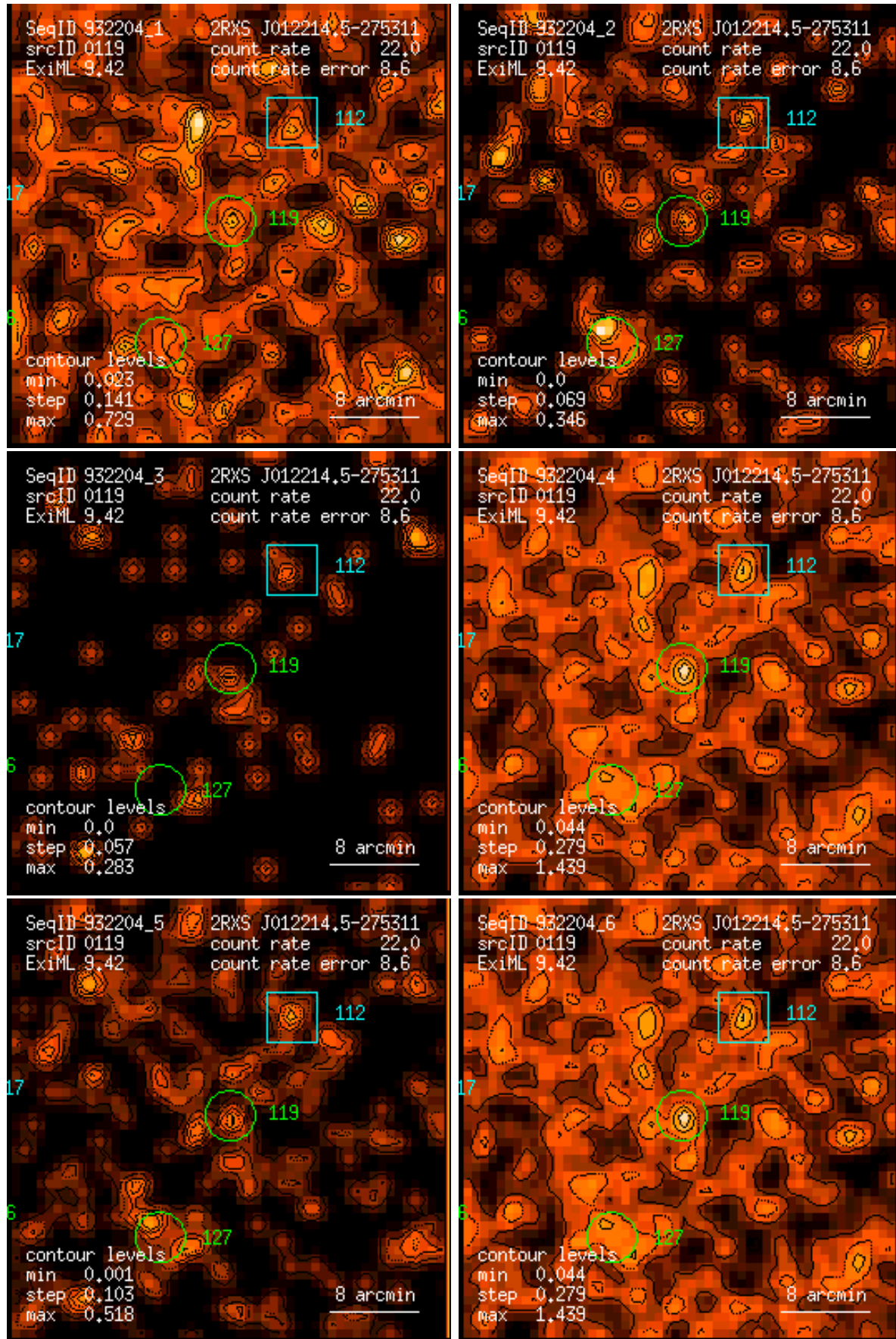
Figure 119: RASS 932204: detection 0119: band rate images, Gaussian filter: (1) PSPC channels 11 – 41, (2) 52 – 90, (3) 91 – 201, (4) 11 – 235, (5) 52 – 201, (6) 11 – 201. Broad band rates in counts/ks. Band rate contour levels in counts/ks/arcmin 2 .
