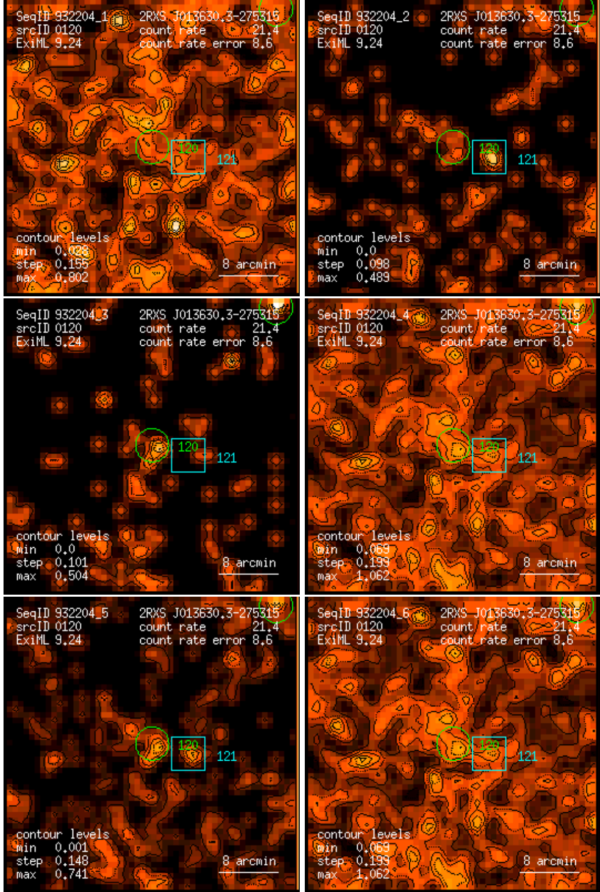
Figure 120: RASS 932204: detection 0120: band rate images, Gaussian filter: (1) PSPC channels 11 – 41, (2) 52 – 90, (3) 91 – 201, (4) 11 – 235, (5) 52 – 201, (6) 11 – 201. Broad band rates in counts/ks. Band rate contour levels in counts/ks/arcmin 2 .
