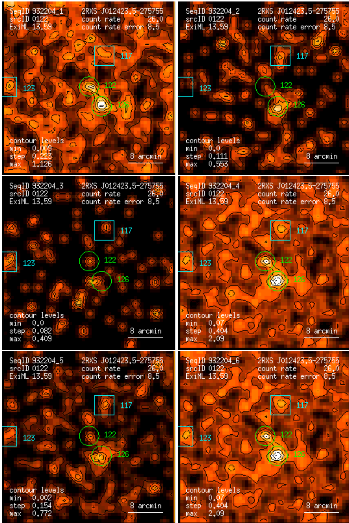
Figure 122: RASS 932204: detection 0122: band rate images, Gaussian filter: (1) PSPC channels 11 – 41, (2) 52 – 90, (3) 91 – 201, (4) 11 – 235, (5) 52 – 201, (6) 11 – 201. Broad band rates in counts/ks. Band rate contour levels in counts/ks/arcmin 2 .
