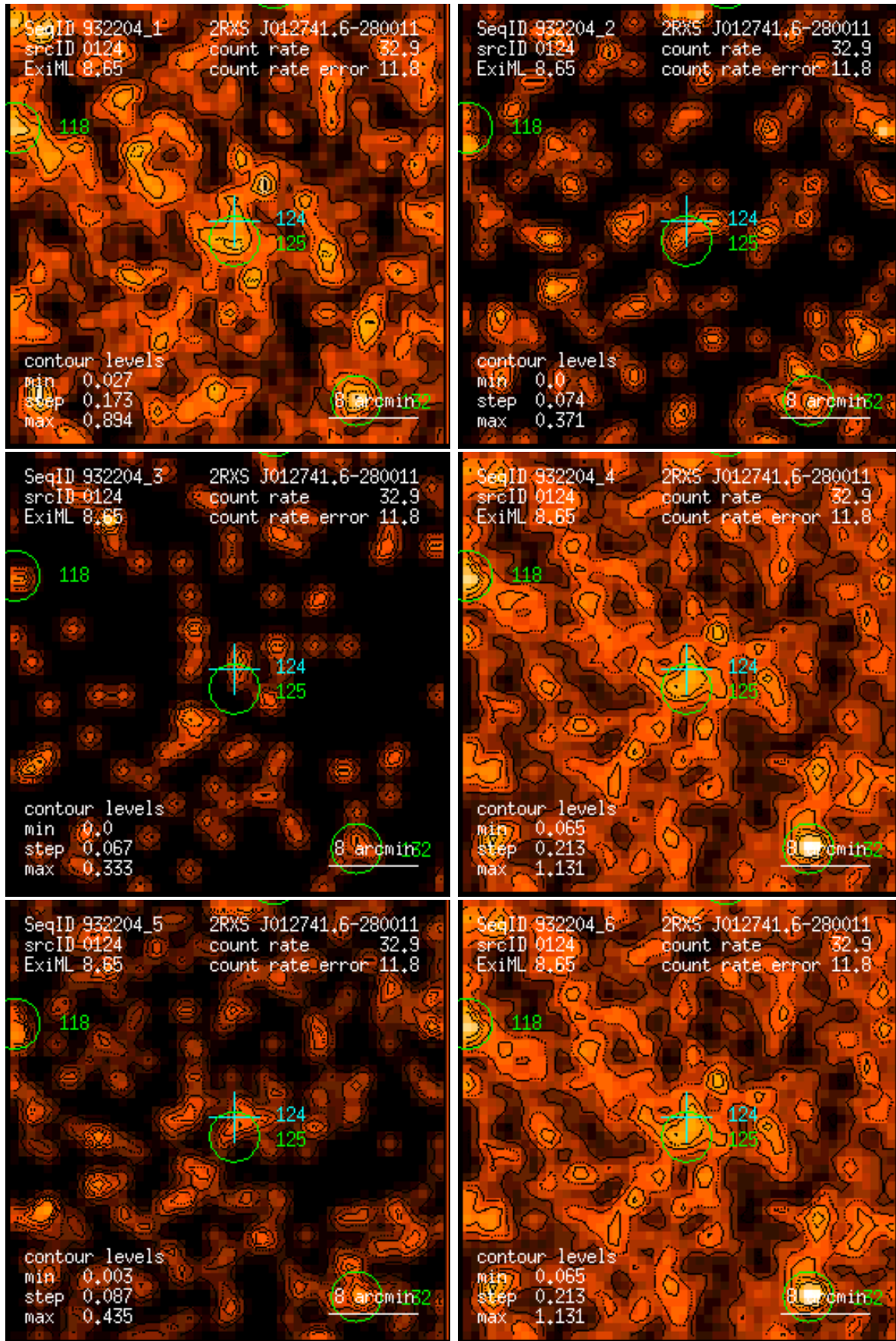
Figure 124: RASS 932204: detection 0124: band rate images, Gaussian filter: (1) PSPC channels 11 – 41, (2) 52 – 90, (3) 91 – 201, (4) 11 – 235, (5) 52 – 201, (6) 11 – 201. Broad band rates in counts/ks. Band rate contour levels in counts/ks/arcmin 2 .
