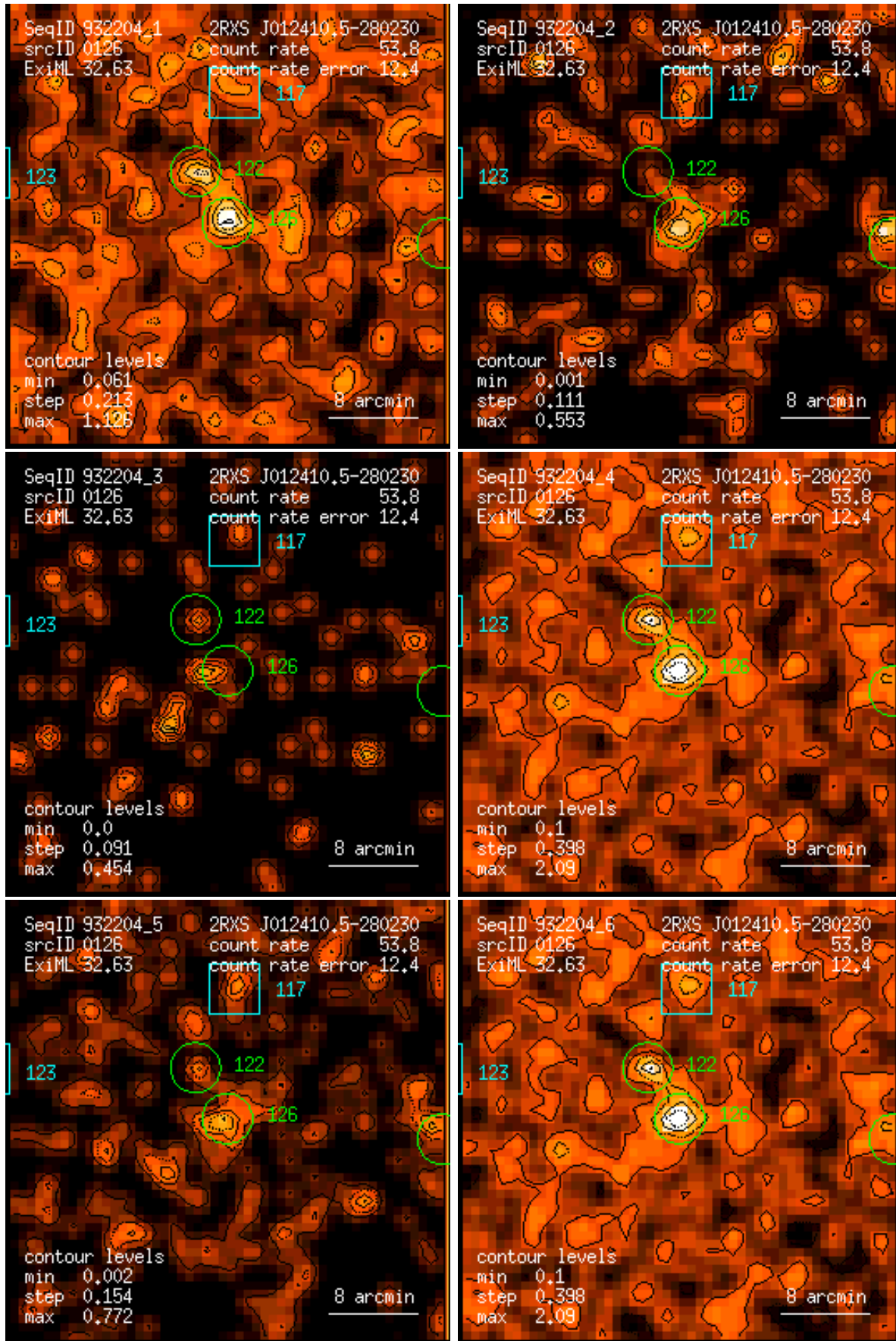
Figure 126: RASS 932204: detection 0126: band rate images, Gaussian filter: (1) PSPC channels 11 – 41, (2) 52 – 90, (3) 91 – 201, (4) 11 – 235, (5) 52 – 201, (6) 11 – 201. Broad band rates in counts/ks. Band rate contour levels in counts/ks/arcmin 2 .
