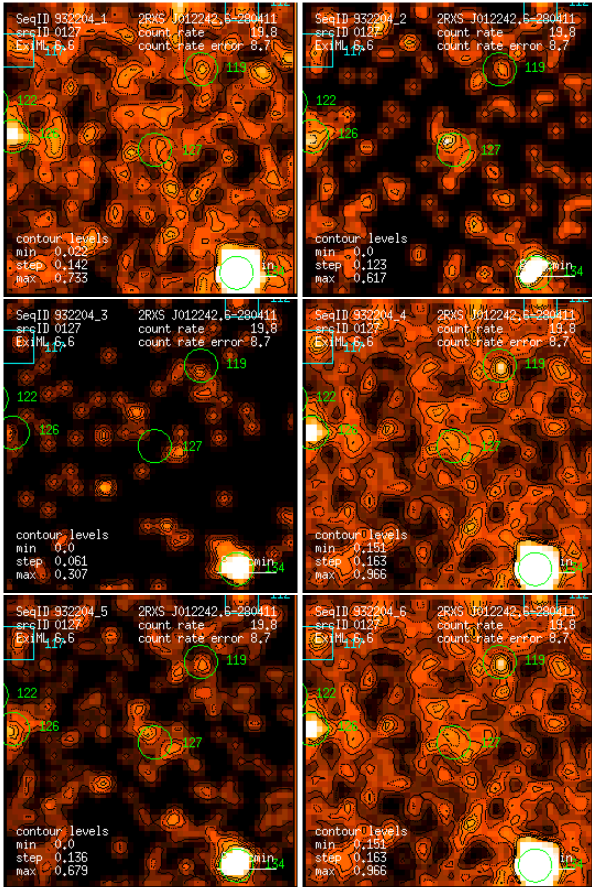
Figure 127: RASS 932204: detection 0127: band rate images, Gaussian filter: (1) PSPC channels 11 – 41, (2) 52 – 90, (3) 91 – 201, (4) 11 – 235, (5) 52 – 201, (6) 11 – 201. Broad band rates in counts/ks. Band rate contour levels in counts/ks/arcmin 2 .
