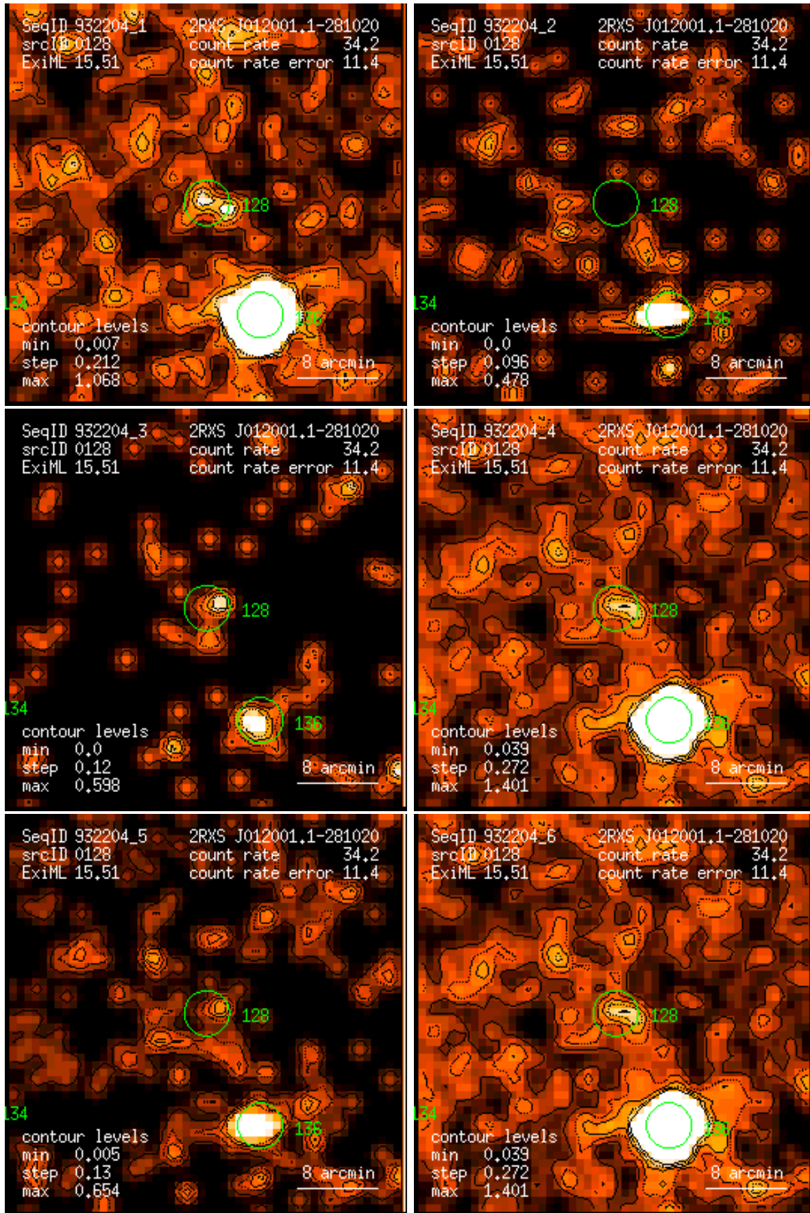
Figure 128: RASS 932204: detection 0128: band rate images, Gaussian filter: (1) PSPC channels 11 – 41, (2) 52 – 90, (3) 91 – 201, (4) 11 – 235, (5) 52 – 201, (6) 11 – 201. Broad band rates in counts/ks. Band rate contour levels in counts/ks/arcmin 2 .
