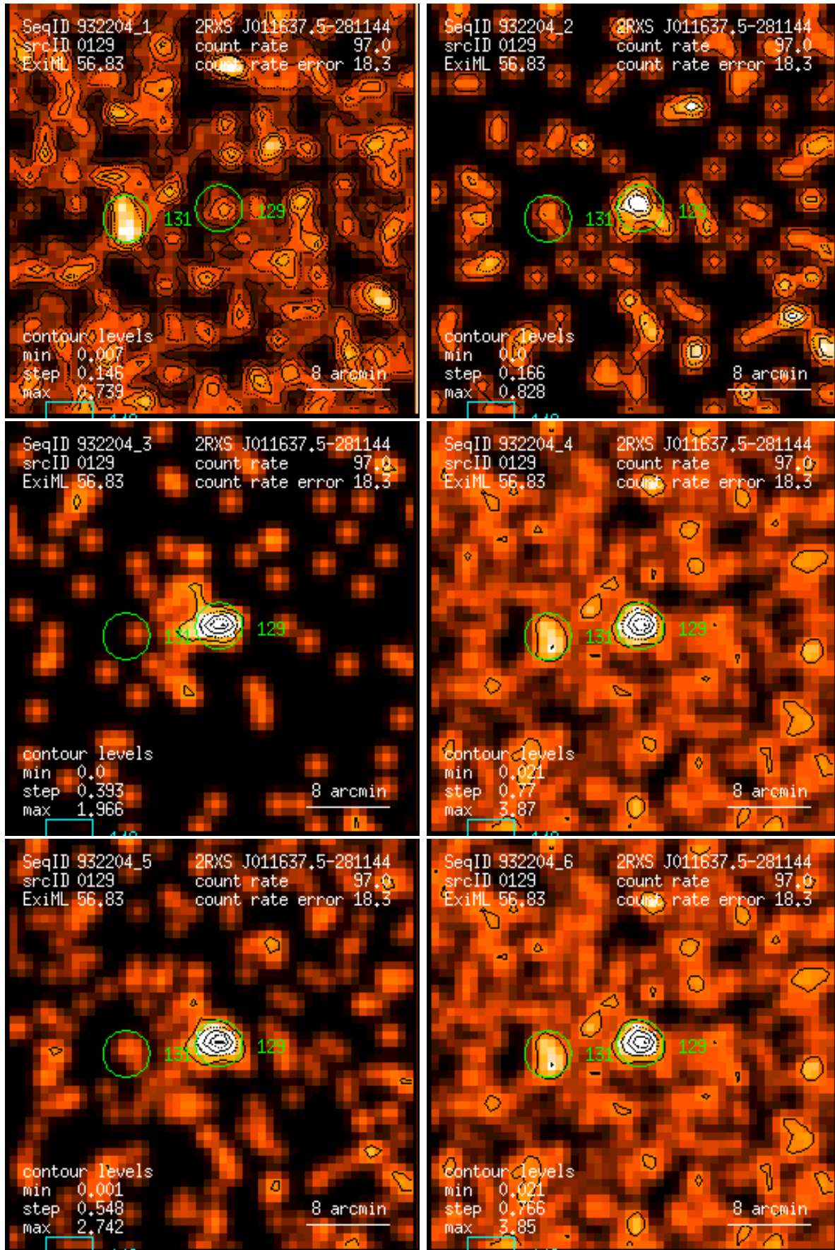
Figure 129: RASS 932204: detection 0129: band rate images, Gaussian filter: (1) PSPC channels 11 – 41, (2) 52 – 90, (3) 91 – 201, (4) 11 – 235, (5) 52 – 201, (6) 11 – 201. Broad band rates in counts/ks. Band rate contour levels in counts/ks/arcmin 2 .
