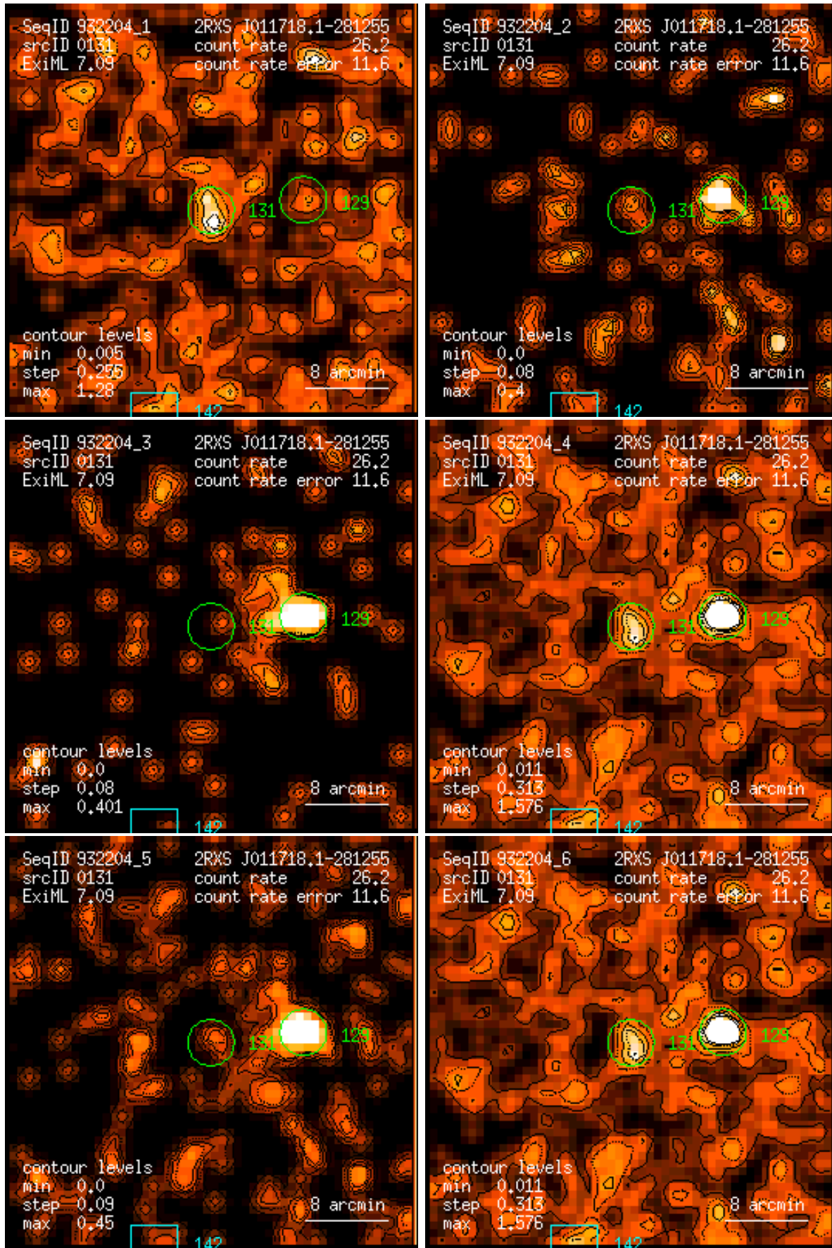
Figure 131: RASS 932204: detection 0131: band rate images, Gaussian filter: (1) PSPC channels 11 – 41, (2) 52 – 90, (3) 91 – 201, (4) 11 – 235, (5) 52 – 201, (6) 11 – 201. Broad band rates in counts/ks. Band rate contour levels in counts/ks/arcmin 2 .
