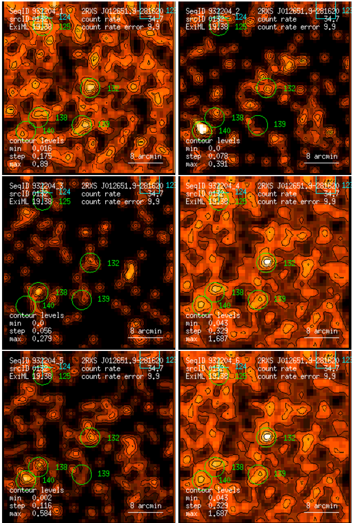
Figure 132: RASS 932204: detection 0132: band rate images, Gaussian filter: (1) PSPC channels 11 – 41, (2) 52 – 90, (3) 91 – 201, (4) 11 – 235, (5) 52 – 201, (6) 11 – 201. Broad band rates in counts/ks. Band rate contour levels in counts/ks/arcmin 2 .
