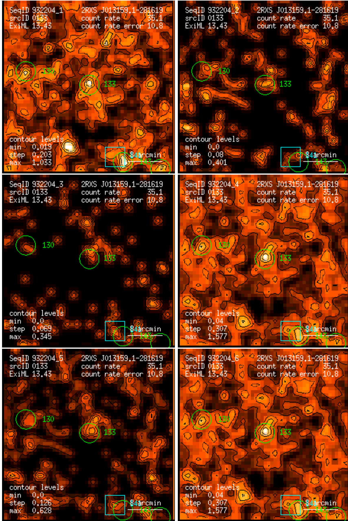
Figure 133: RASS 932204: detection 0133: band rate images, Gaussian filter: (1) PSPC channels 11 – 41, (2) 52 – 90, (3) 91 – 201, (4) 11 – 235, (5) 52 – 201, (6) 11 – 201. Broad band rates in counts/ks. Band rate contour levels in counts/ks/arcmin 2 .
