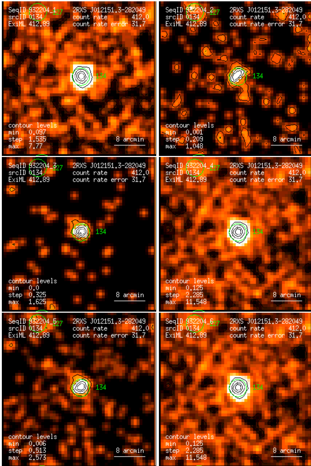
Figure 134: RASS 932204: detection 0134: band rate images, Gaussian filter: (1) PSPC channels 11 – 41, (2) 52 – 90, (3) 91 – 201, (4) 11 – 235, (5) 52 – 201, (6) 11 – 201. Broad band rates in counts/ks. Band rate contour levels in counts/ks/arcmin 2 .
