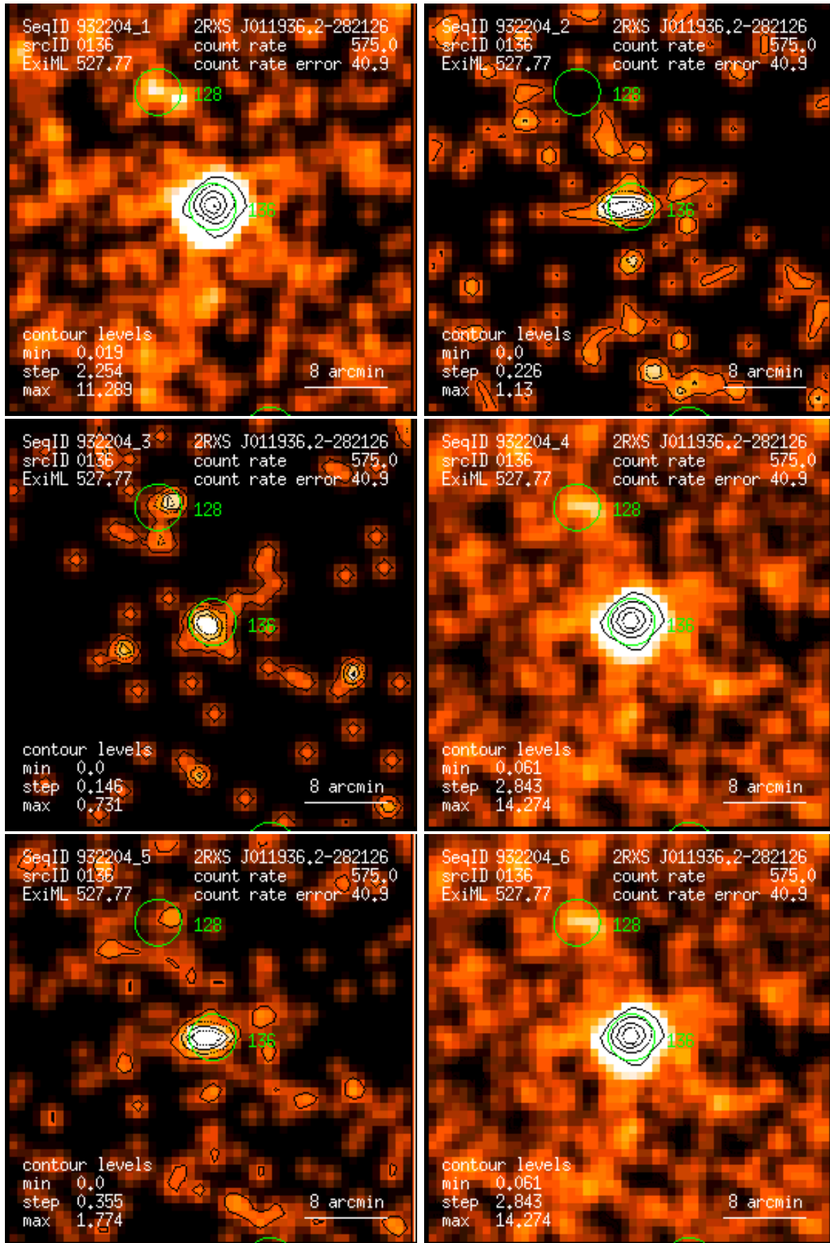
Figure 136: RASS 932204: detection 0136: band rate images, Gaussian filter: (1) PSPC channels 11 – 41, (2) 52 – 90, (3) 91 – 201, (4) 11 – 235, (5) 52 – 201, (6) 11 – 201. Broad band rates in counts/ks. Band rate contour levels in counts/ks/arcmin 2 .
