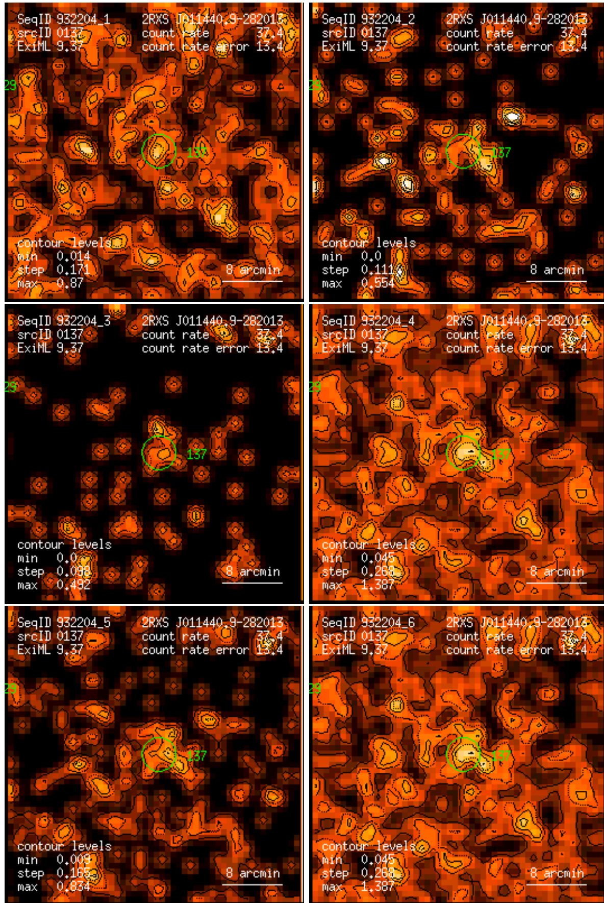
Figure 137: RASS 932204: detection 0137: band rate images, Gaussian filter: (1) PSPC channels 11 – 41, (2) 52 – 90, (3) 91 – 201, (4) 11 – 235, (5) 52 – 201, (6) 11 – 201. Broad band rates in counts/ks. Band rate contour levels in counts/ks/arcmin 2 .
