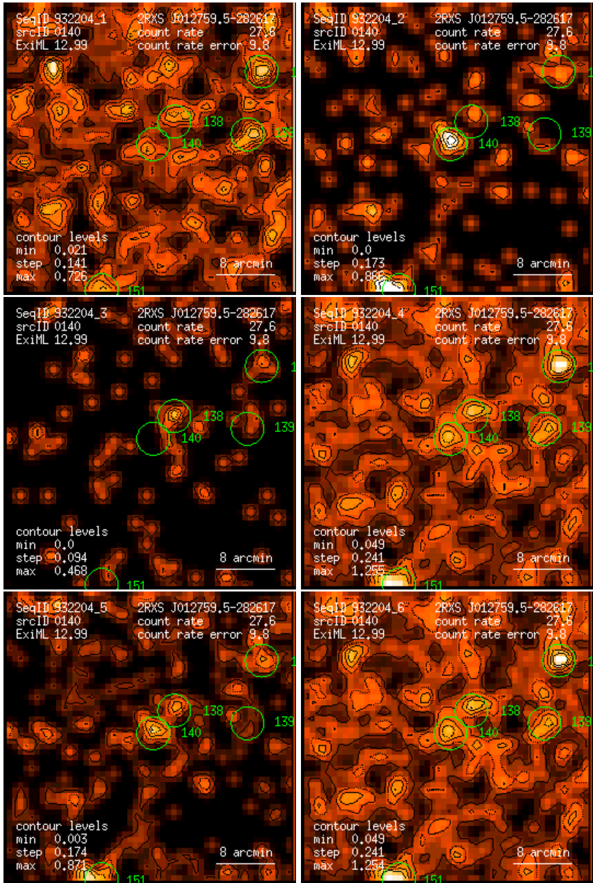
Figure 140: RASS 932204: detection 0140: band rate images, Gaussian filter: (1) PSPC channels 11 – 41, (2) 52 – 90, (3) 91 – 201, (4) 11 – 235, (5) 52 – 201, (6) 11 – 201. Broad band rates in counts/ks. Band rate contour levels in counts/ks/arcmin 2 .
