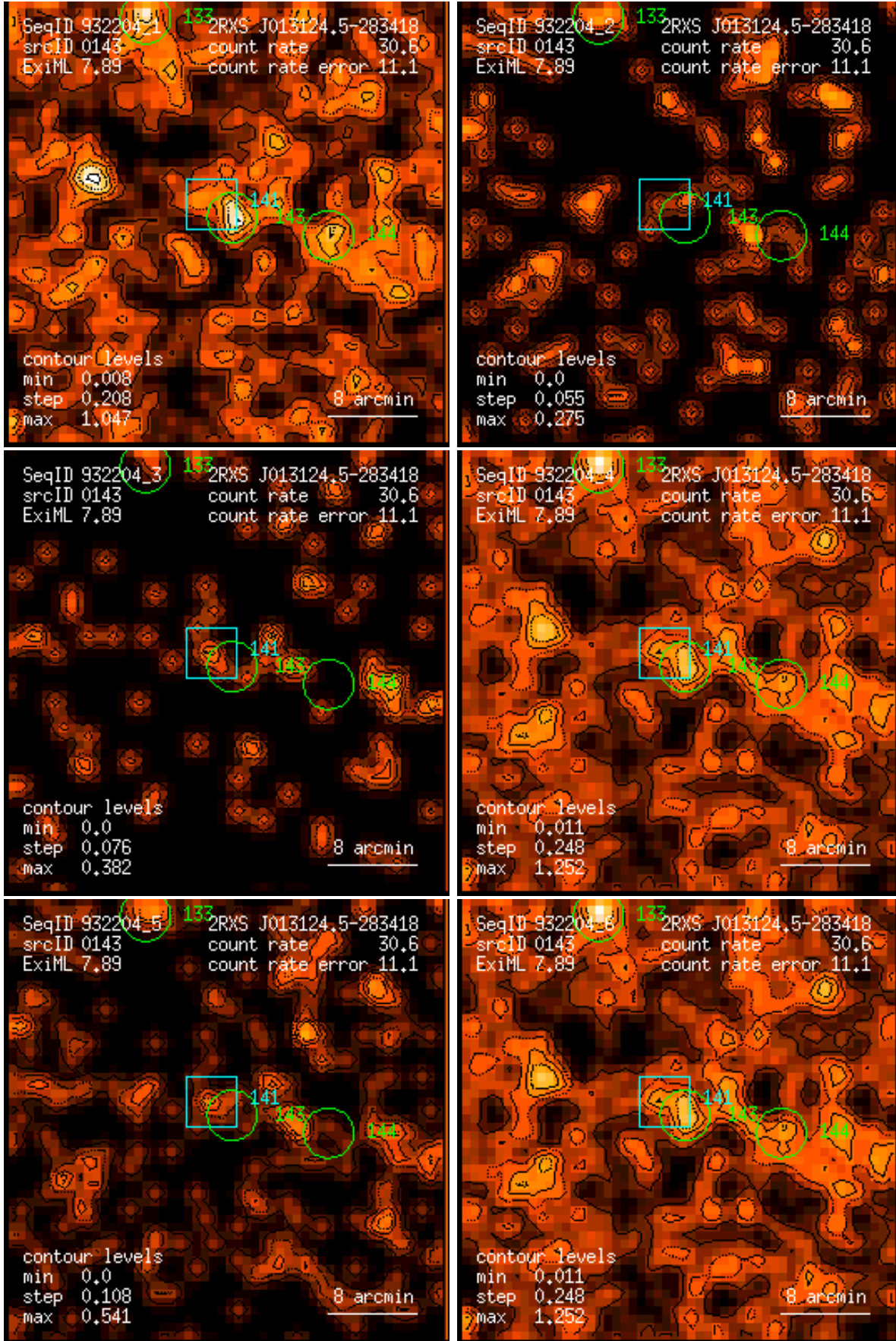
Figure 143: RASS 932204: detection 0143: band rate images, Gaussian filter: (1) PSPC channels 11 – 41, (2) 52 – 90, (3) 91 – 201, (4) 11 – 235, (5) 52 – 201, (6) 11 – 201. Broad band rates in counts/ks. Band rate contour levels in counts/ks/arcmin 2 .
