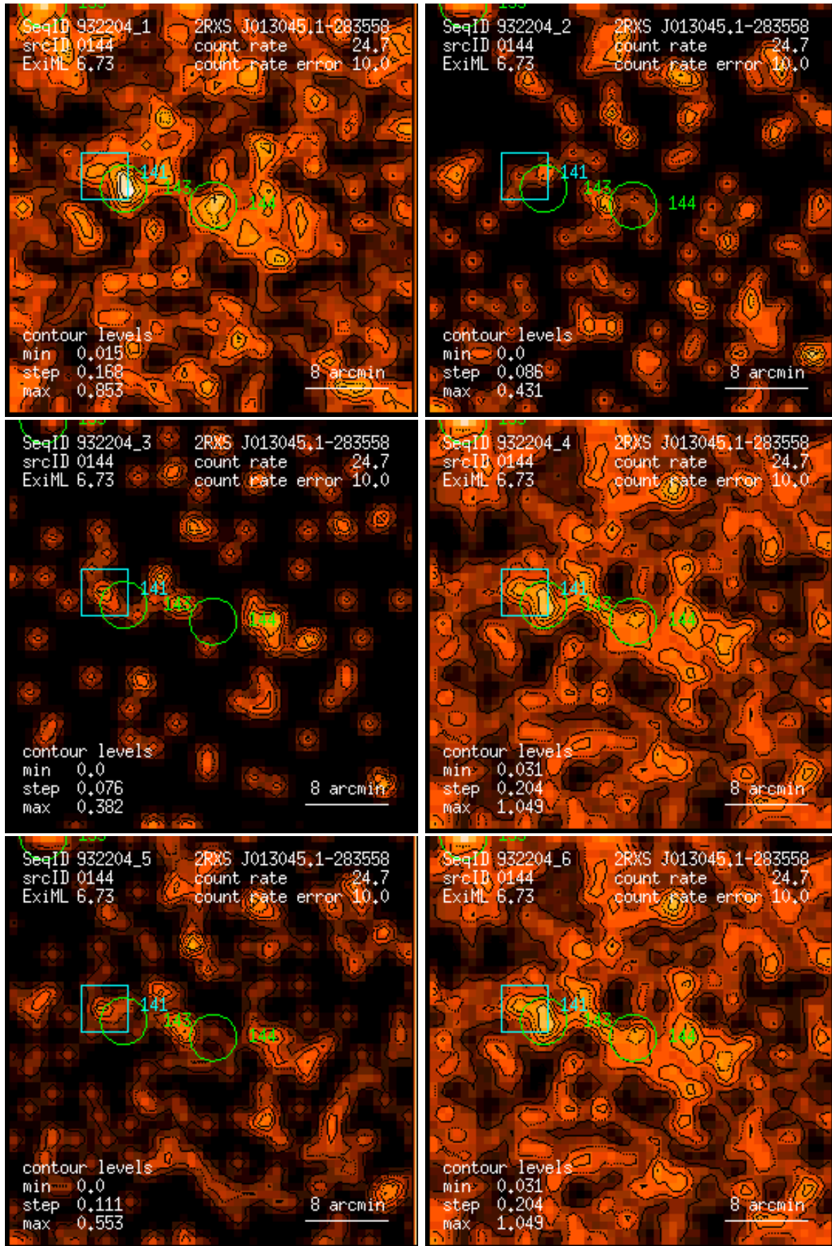
Figure 144: RASS 932204: detection 0144: band rate images, Gaussian filter: (1) PSPC channels 11 – 41, (2) 52 – 90, (3) 91 – 201, (4) 11 – 235, (5) 52 – 201, (6) 11 – 201. Broad band rates in counts/ks. Band rate contour levels in counts/ks/arcmin 2 .
