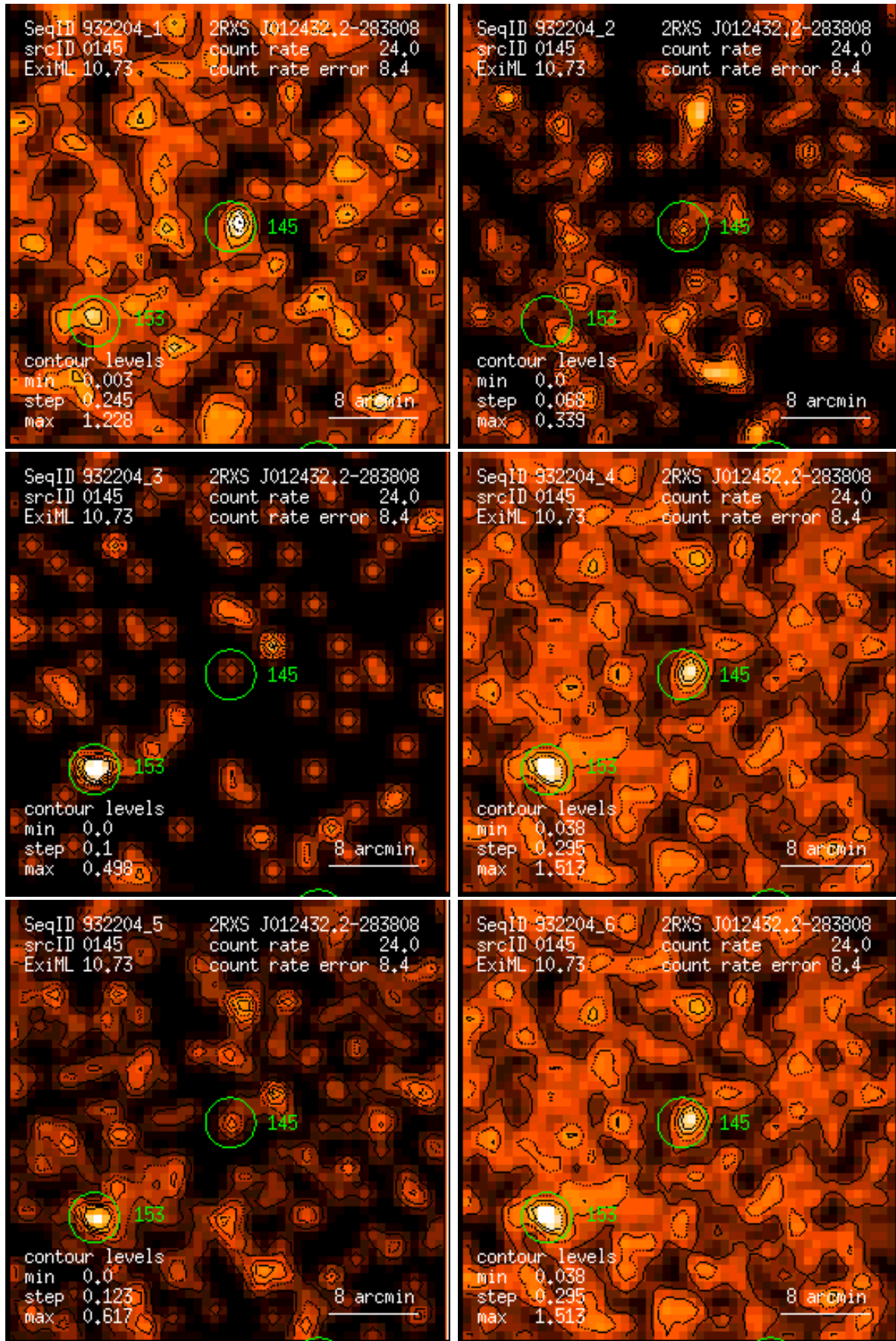
Figure 145: RASS 932204: detection 0145: band rate images, Gaussian filter: (1) PSPC channels 11 – 41, (2) 52 – 90, (3) 91 – 201, (4) 11 – 235, (5) 52 – 201, (6) 11 – 201. Broad band rates in counts/ks. Band rate contour levels in counts/ks/arcmin 2 .
