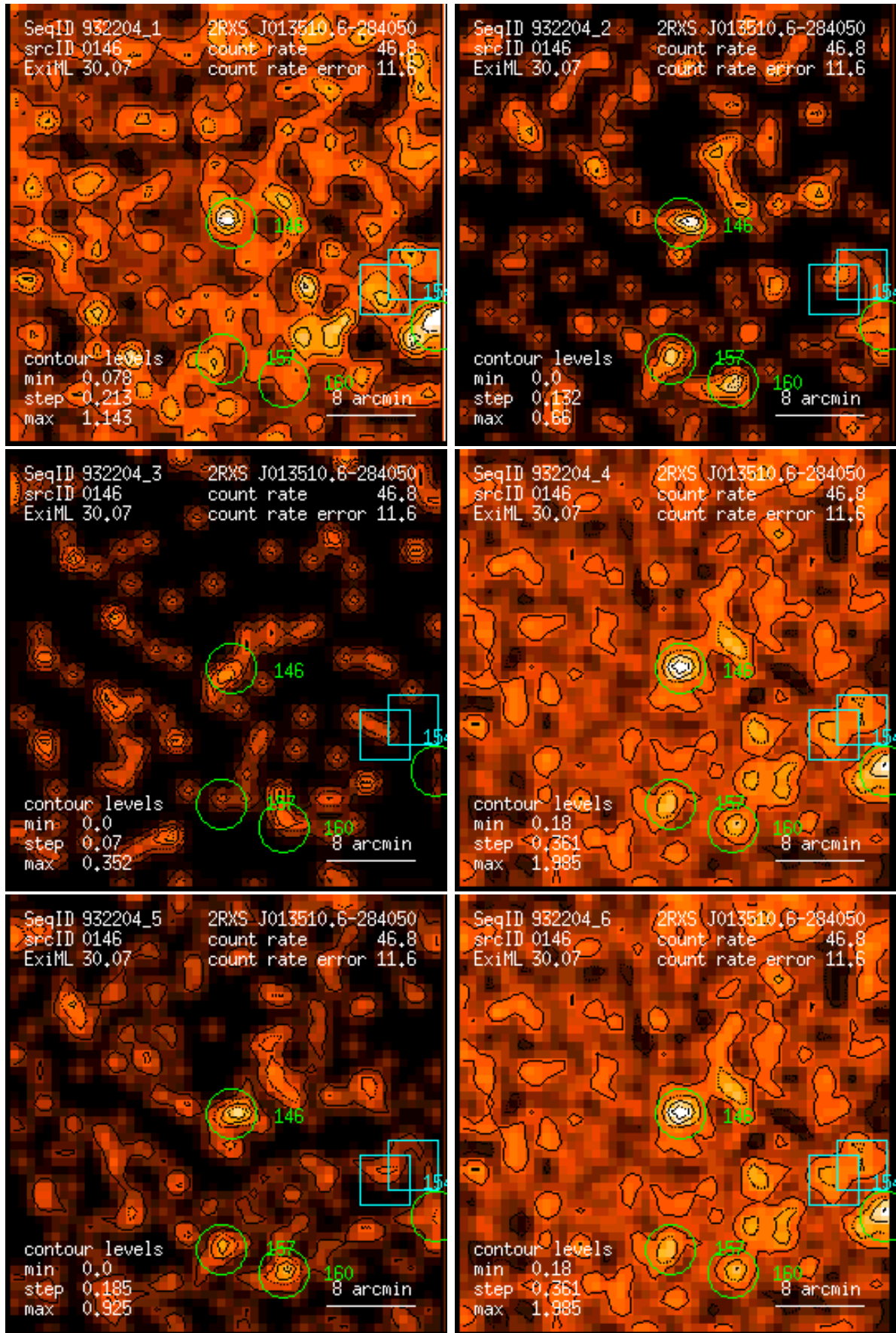
Figure 146: RASS 932204: detection 0146: band rate images, Gaussian filter: (1) PSPC channels 11 – 41, (2) 52 – 90, (3) 91 – 201, (4) 11 – 235, (5) 52 – 201, (6) 11 – 201. Broad band rates in counts/ks. Band rate contour levels in counts/ks/arcmin 2 .
