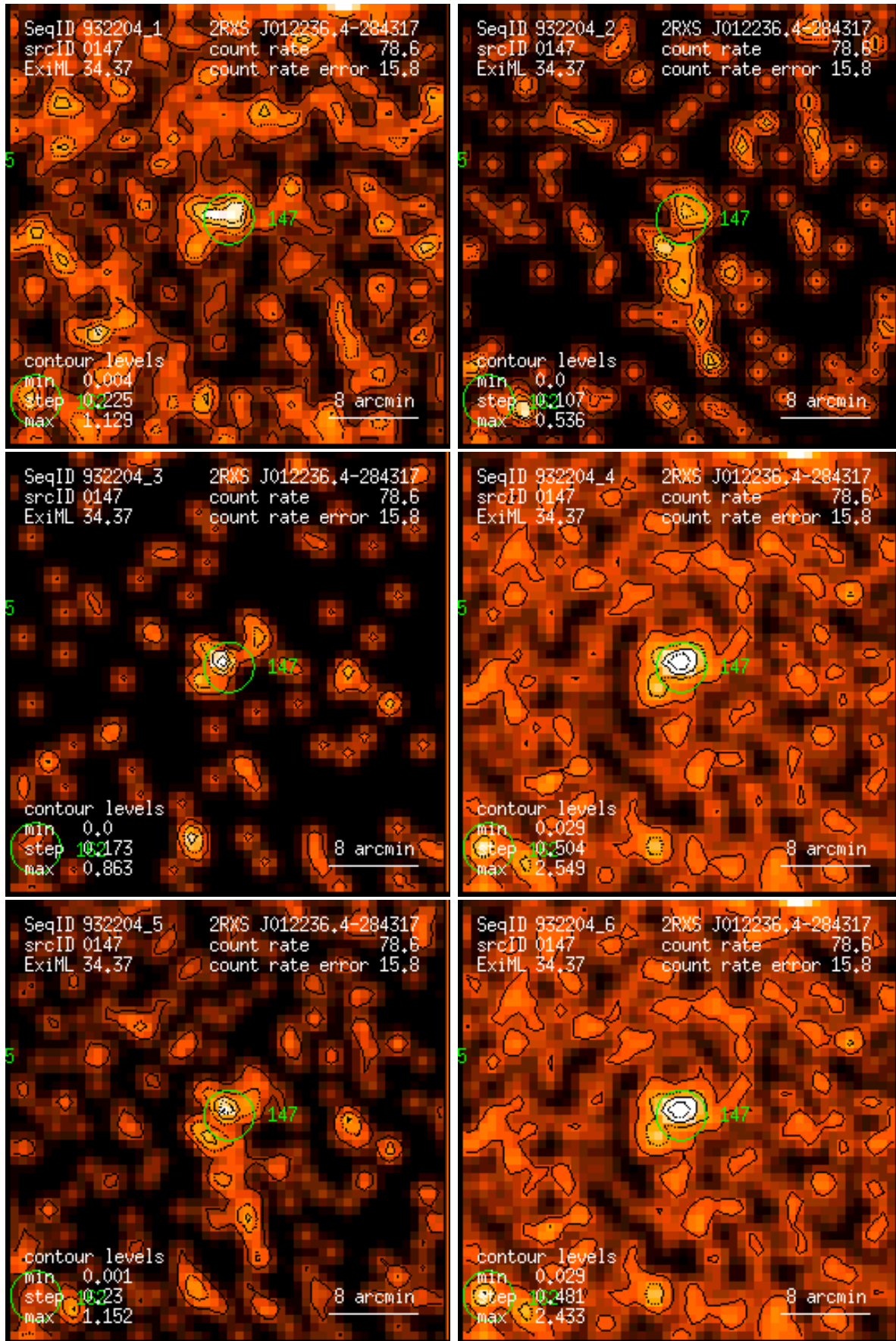
Figure 147: RASS 932204: detection 0147: band rate images, Gaussian filter: (1) PSPC channels 11 – 41, (2) 52 – 90, (3) 91 – 201, (4) 11 – 235, (5) 52 – 201, (6) 11 – 201. Broad band rates in counts/ks. Band rate contour levels in counts/ks/arcmin 2 .
