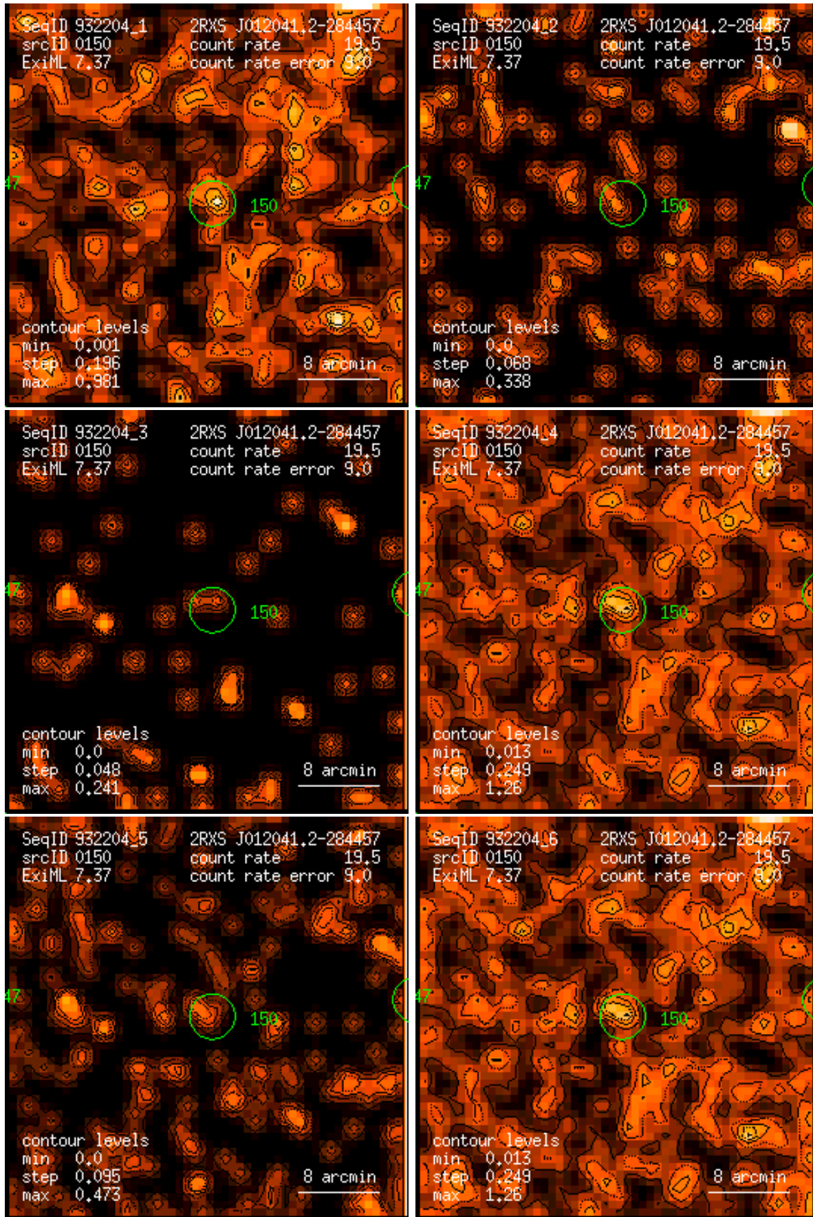
Figure 150: RASS 932204: detection 0150: band rate images, Gaussian filter: (1) PSPC channels 11 – 41, (2) 52 – 90, (3) 91 – 201, (4) 11 – 235, (5) 52 – 201, (6) 11 – 201. Broad band rates in counts/ks. Band rate contour levels in counts/ks/arcmin 2 .
