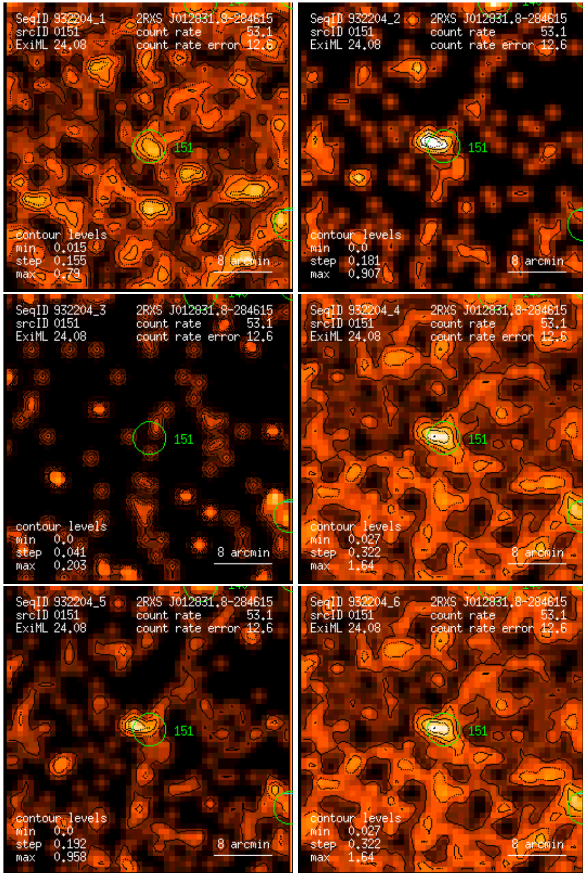
Figure 151: RASS 932204: detection 0151: band rate images, Gaussian filter: (1) PSPC channels 11 – 41, (2) 52 – 90, (3) 91 – 201, (4) 11 – 235, (5) 52 – 201, (6) 11 – 201. Broad band rates in counts/ks. Band rate contour levels in counts/ks/arcmin 2 .
