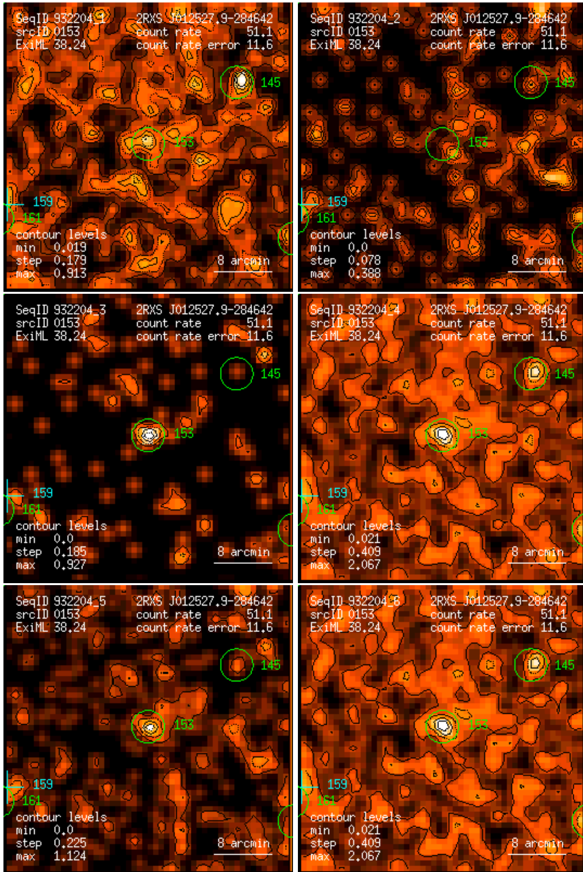
Figure 153: RASS 932204: detection 0153: band rate images, Gaussian filter: (1) PSPC channels 11 – 41, (2) 52 – 90, (3) 91 – 201, (4) 11 – 235, (5) 52 – 201, (6) 11 – 201. Broad band rates in counts/ks. Band rate contour levels in counts/ks/arcmin 2 .
