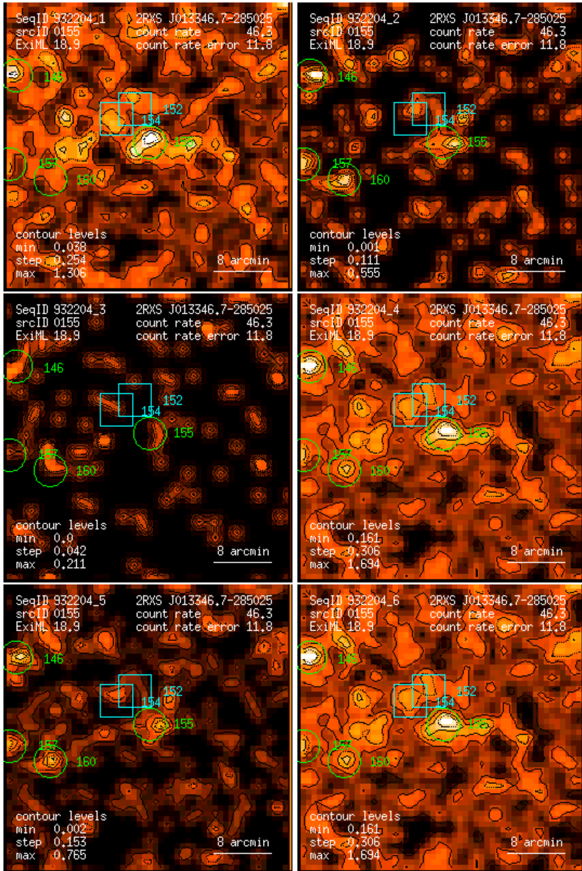
Figure 155: RASS 932204: detection 0155: band rate images, Gaussian filter: (1) PSPC channels 11 – 41, (2) 52 – 90, (3) 91 – 201, (4) 11 – 235, (5) 52 – 201, (6) 11 – 201. Broad band rates in counts/ks. Band rate contour levels in counts/ks/arcmin 2 .
