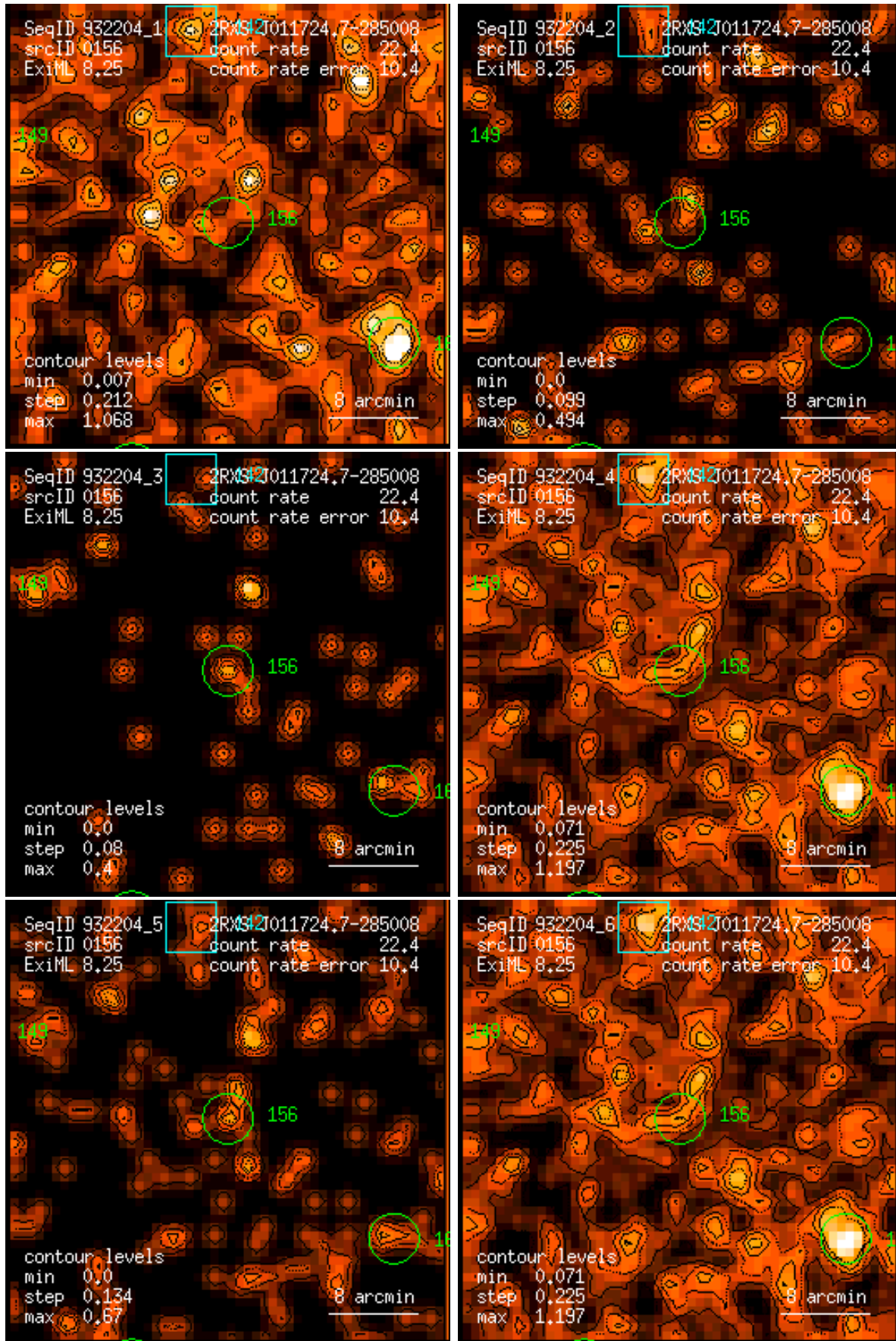
Figure 156: RASS 932204: detection 0156: band rate images, Gaussian filter: (1) PSPC channels 11 – 41, (2) 52 – 90, (3) 91 – 201, (4) 11 – 235, (5) 52 – 201, (6) 11 – 201. Broad band rates in counts/ks. Band rate contour levels in counts/ks/arcmin 2 .
