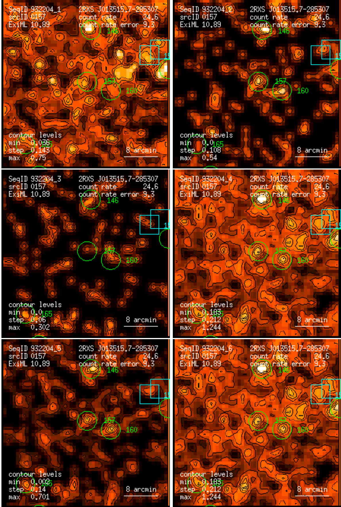
Figure 157: RASS 932204: detection 0157: band rate images, Gaussian filter: (1) PSPC channels 11 – 41, (2) 52 – 90, (3) 91 – 201, (4) 11 – 235, (5) 52 – 201, (6) 11 – 201. Broad band rates in counts/ks. Band rate contour levels in counts/ks/arcmin 2 .
