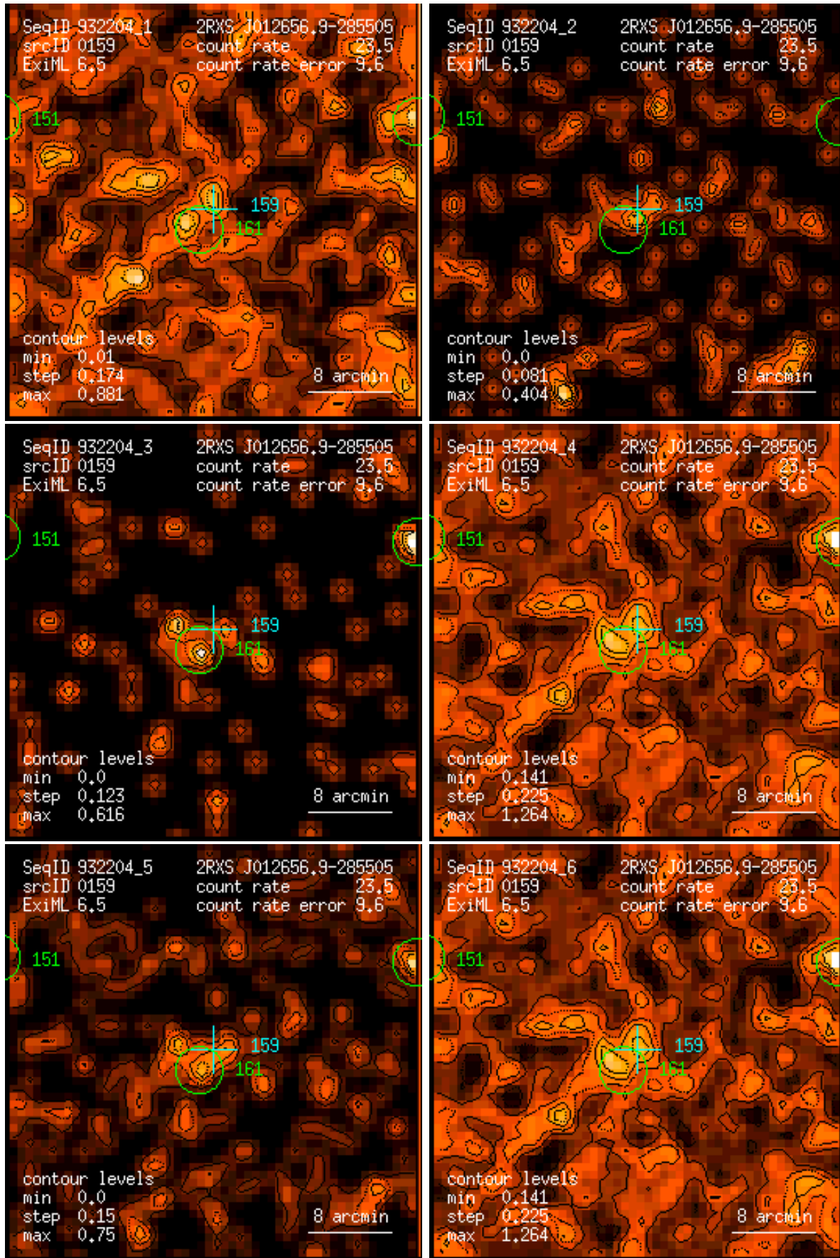
Figure 159: RASS 932204: detection 0159: band rate images, Gaussian filter: (1) PSPC channels 11 – 41, (2) 52 – 90, (3) 91 – 201, (4) 11 – 235, (5) 52 – 201, (6) 11 – 201. Broad band rates in counts/ks. Band rate contour levels in counts/ks/arcmin 2 .
