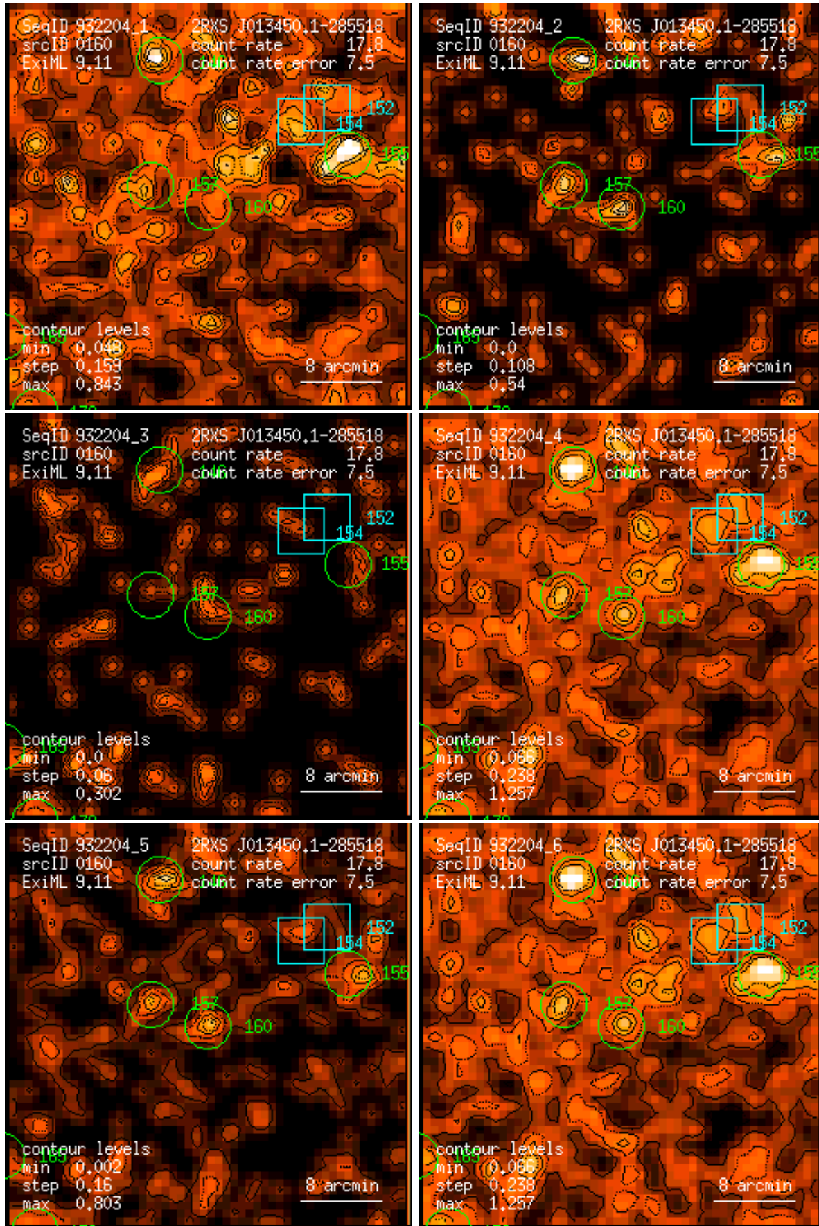
Figure 160: RASS 932204: detection 0160: band rate images, Gaussian filter: (1) PSPC channels 11 – 41, (2) 52 – 90, (3) 91 – 201, (4) 11 – 235, (5) 52 – 201, (6) 11 – 201. Broad band rates in counts/ks. Band rate contour levels in counts/ks/arcmin 2 .
