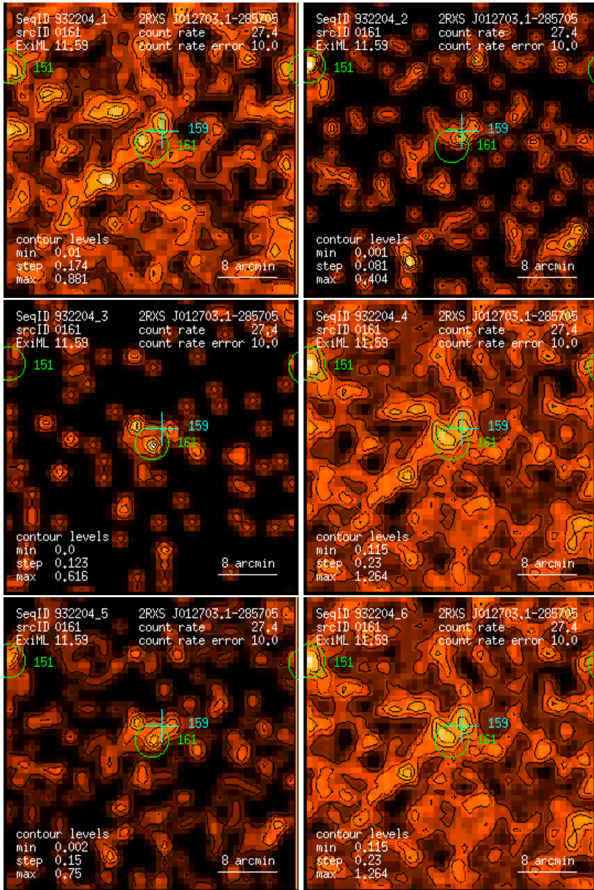
Figure 161: RASS 932204: detection 0161: band rate images, Gaussian filter: (1) PSPC channels 11 – 41, (2) 52 – 90, (3) 91 – 201, (4) 11 – 235, (5) 52 – 201, (6) 11 – 201. Broad band rates in counts/ks. Band rate contour levels in counts/ks/arcmin 2 .
