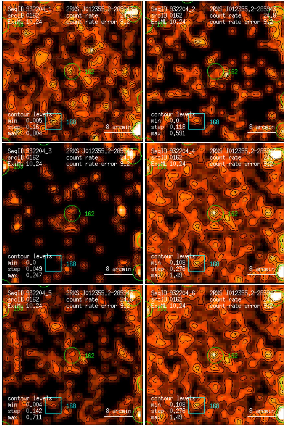
Figure 162: RASS 932204: detection 0162: band rate images, Gaussian filter: (1) PSPC channels 11 – 41, (2) 52 – 90, (3) 91 – 201, (4) 11 – 235, (5) 52 – 201, (6) 11 – 201. Broad band rates in counts/ks. Band rate contour levels in counts/ks/arcmin 2 .
