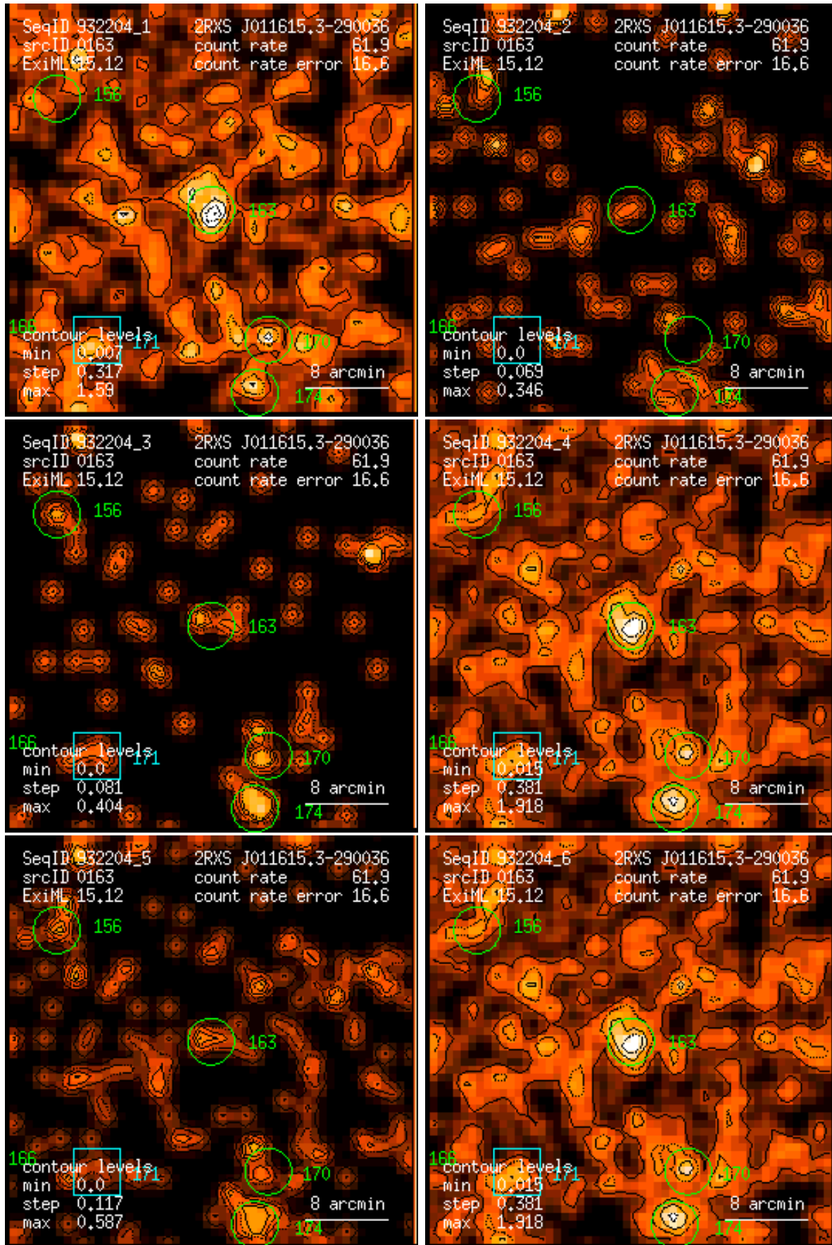
Figure 163: RASS 932204: detection 0163: band rate images, Gaussian filter: (1) PSPC channels 11 – 41, (2) 52 – 90, (3) 91 – 201, (4) 11 – 235, (5) 52 – 201, (6) 11 – 201. Broad band rates in counts/ks. Band rate contour levels in counts/ks/arcmin 2 .
