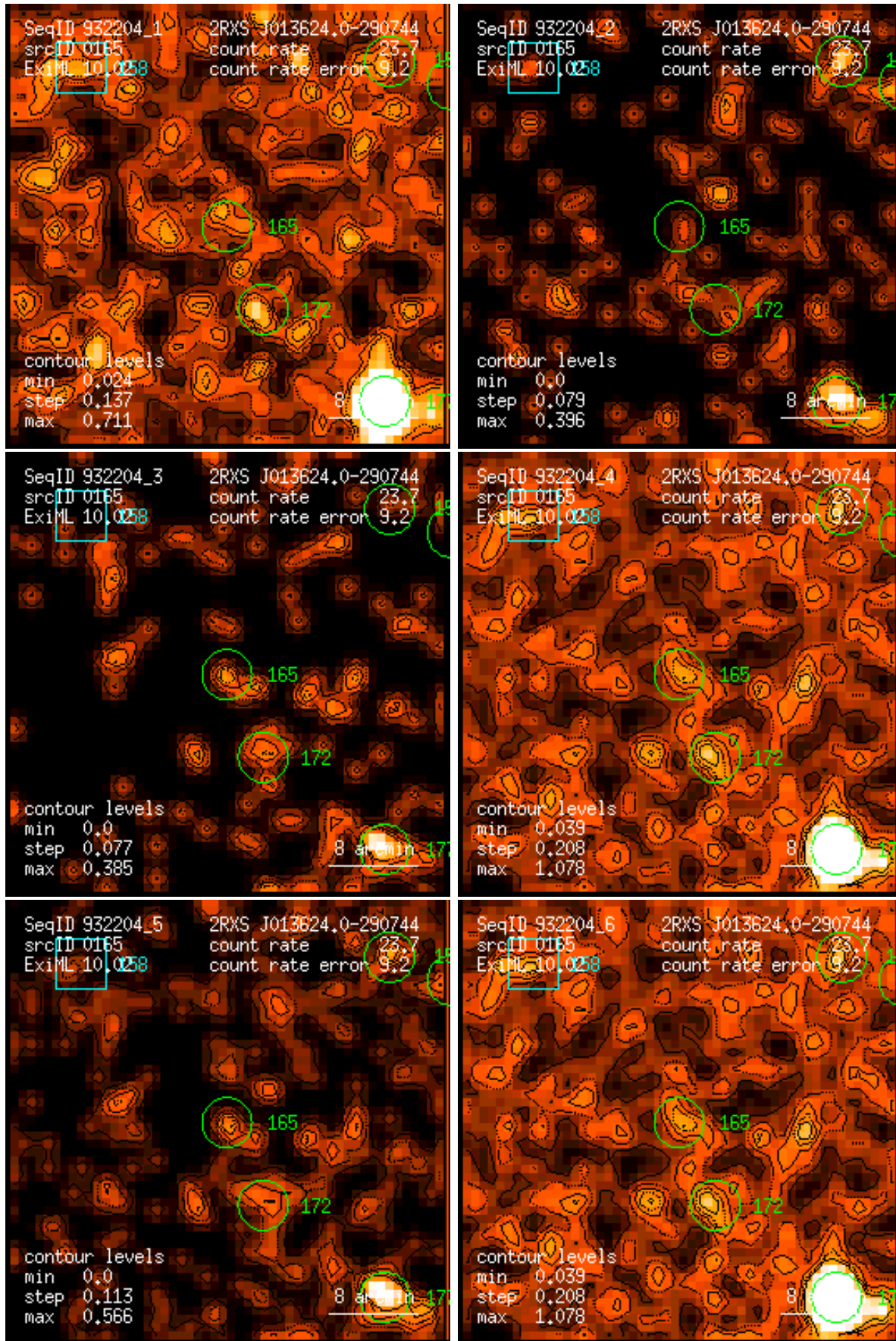
Figure 165: RASS 932204: detection 0165: band rate images, Gaussian filter: (1) PSPC channels 11 – 41, (2) 52 – 90, (3) 91 – 201, (4) 11 – 235, (5) 52 – 201, (6) 11 – 201. Broad band rates in counts/ks. Band rate contour levels in counts/ks/arcmin 2 .
