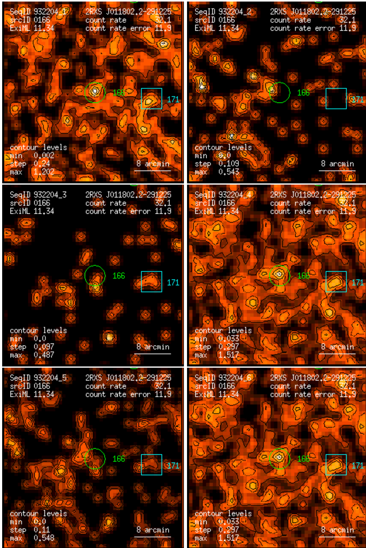
Figure 166: RASS 932204: detection 0166: band rate images, Gaussian filter: (1) PSPC channels 11 – 41, (2) 52 – 90, (3) 91 – 201, (4) 11 – 235, (5) 52 – 201, (6) 11 – 201. Broad band rates in counts/ks. Band rate contour levels in counts/ks/arcmin 2 .
