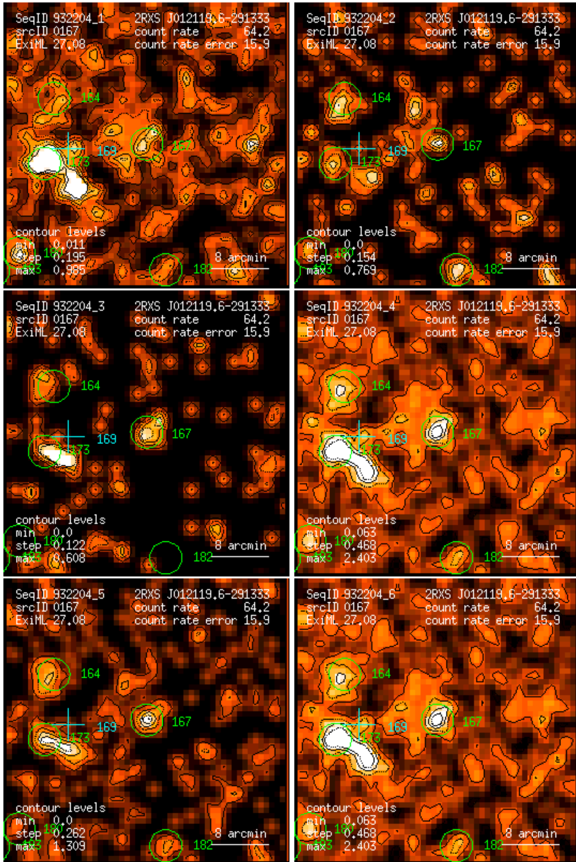
Figure 167: RASS 932204: detection 0167: band rate images, Gaussian filter: (1) PSPC channels 11 – 41, (2) 52 – 90, (3) 91 – 201, (4) 11 – 235, (5) 52 – 201, (6) 11 – 201. Broad band rates in counts/ks. Band rate contour levels in counts/ks/arcmin 2 .
