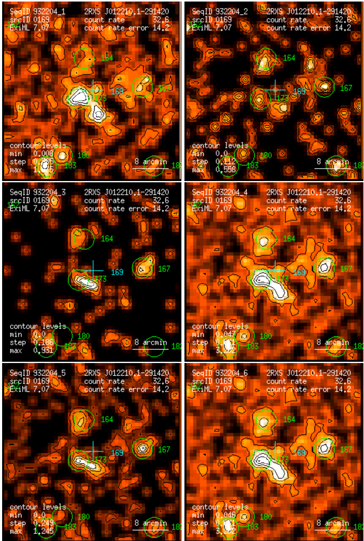
Figure 169: RASS 932204: detection 0169: band rate images, Gaussian filter: (1) PSPC channels 11 – 41, (2) 52 – 90, (3) 91 – 201, (4) 11 – 235, (5) 52 – 201, (6) 11 – 201. Broad band rates in counts/ks. Band rate contour levels in counts/ks/arcmin 2 .
