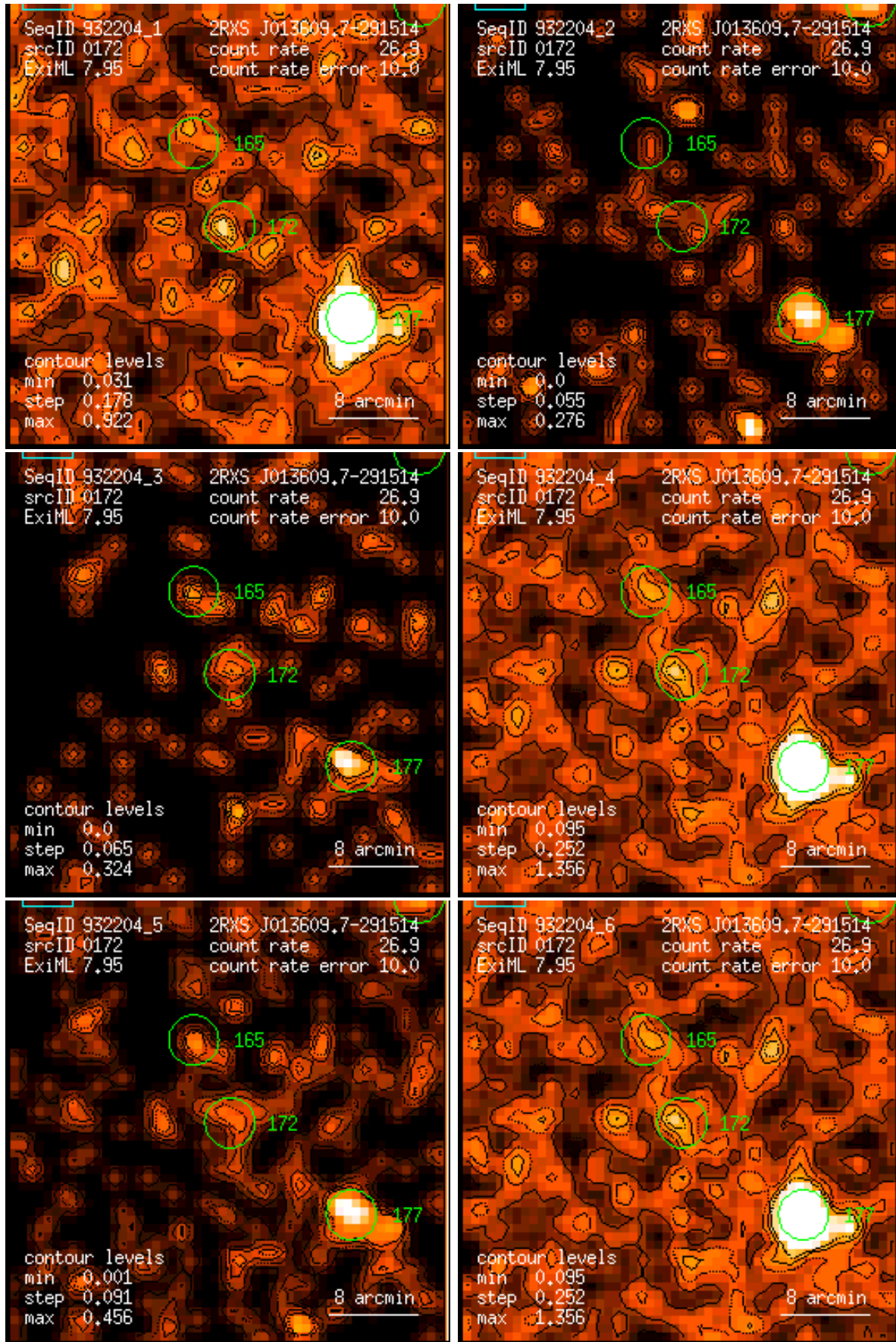
Figure 172: RASS 932204: detection 0172: band rate images, Gaussian filter: (1) PSPC channels 11 – 41, (2) 52 – 90, (3) 91 – 201, (4) 11 – 235, (5) 52 – 201, (6) 11 – 201. Broad band rates in counts/ks. Band rate contour levels in counts/ks/arcmin 2 .
